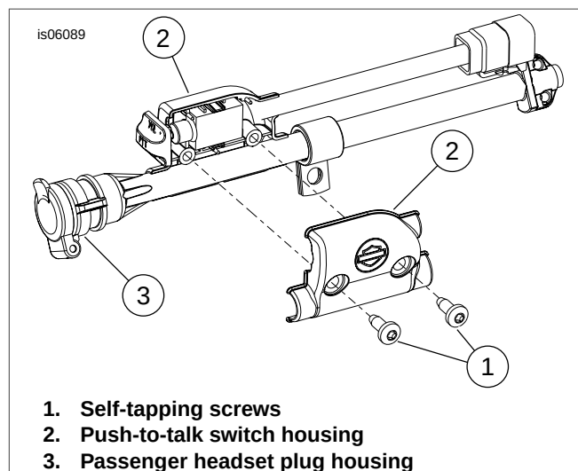
Figure 1. Install Push-to-Talk Switch Housing
