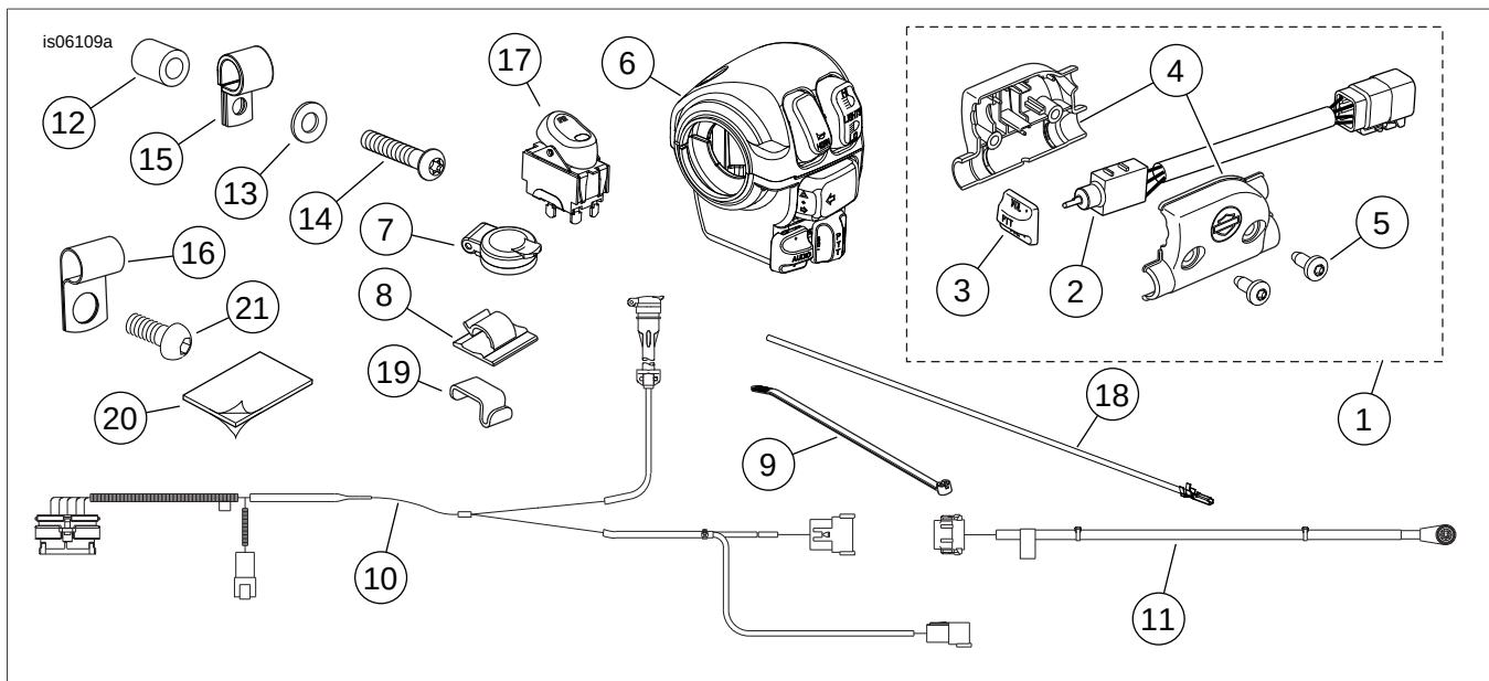
Figure 7. Service Parts, Music and Intercom Kit
