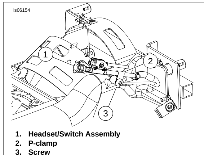
Figure 4. Installation on Trikes Without Tour-Pak
