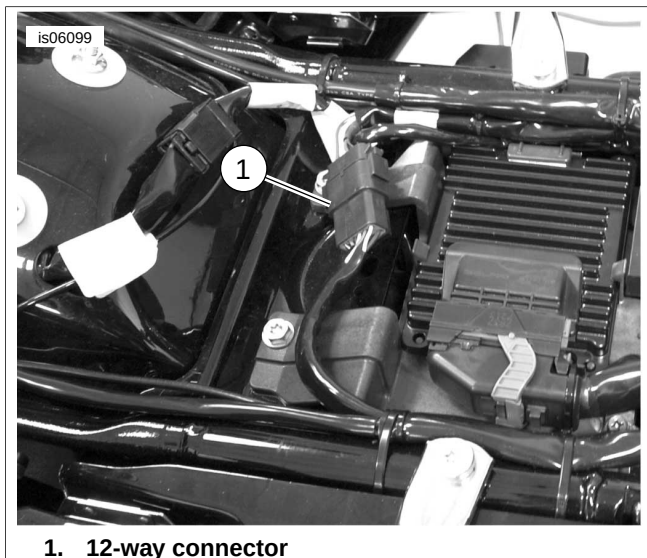
Figure 5. 12-Way Connector of Overlay Harness
