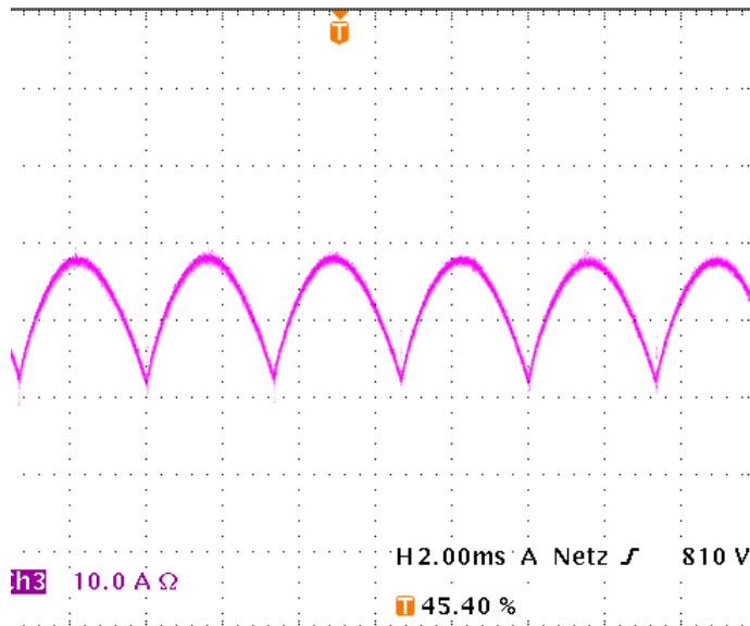
Six current pulses in positive direction
