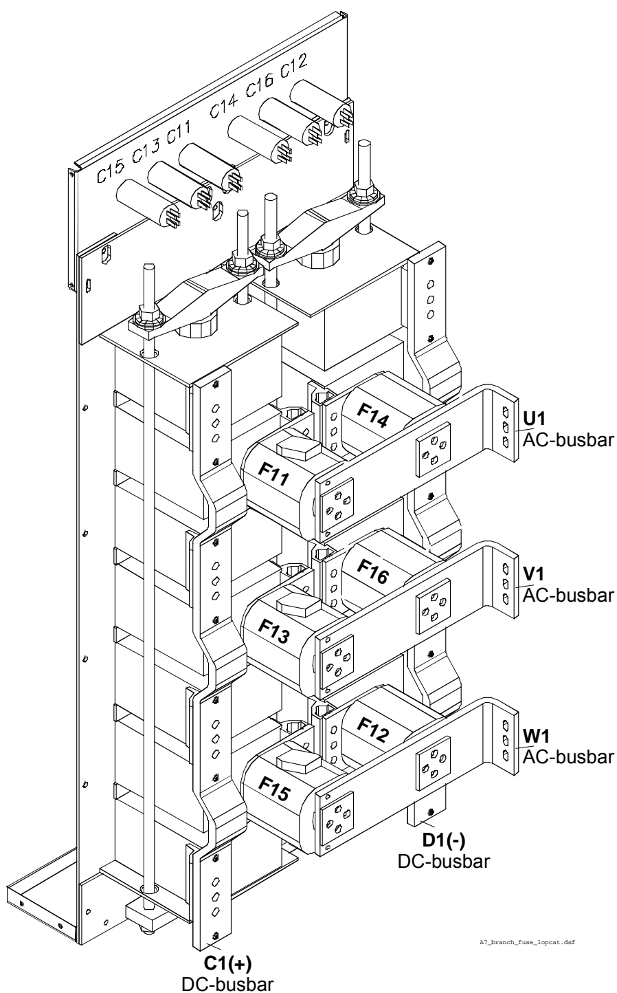
Location of branch fuses frame D7 (busbars on the right)
