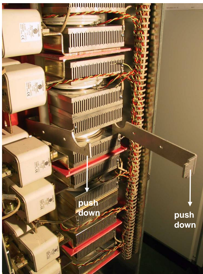
Use of disassembly tool
