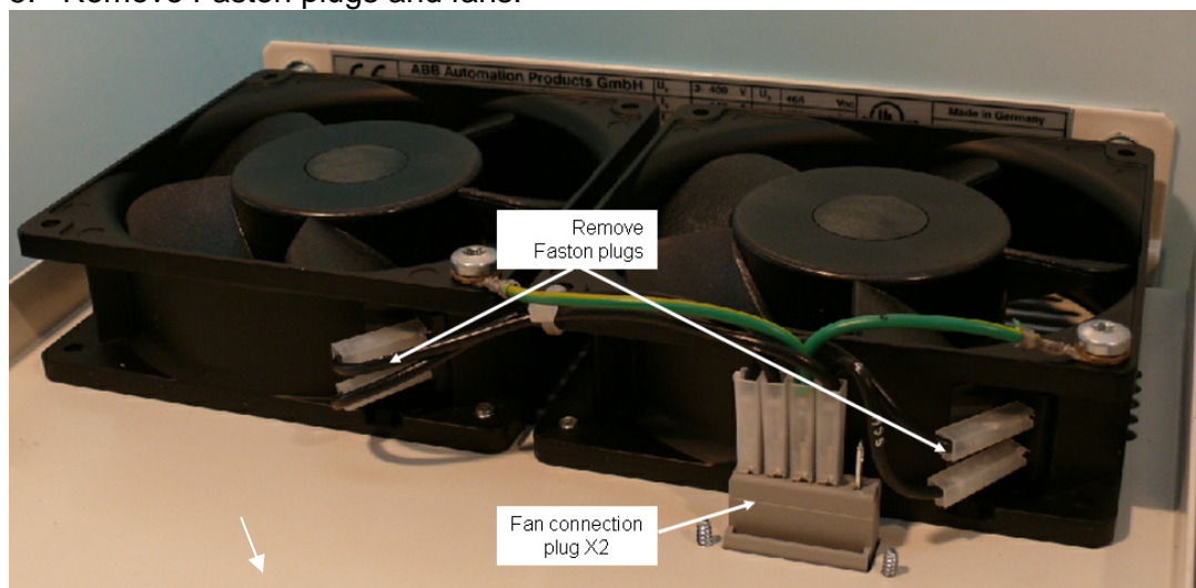
Faston plugs
