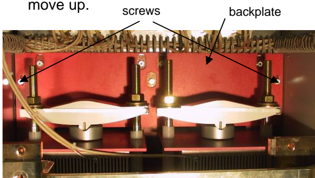
Backplate
