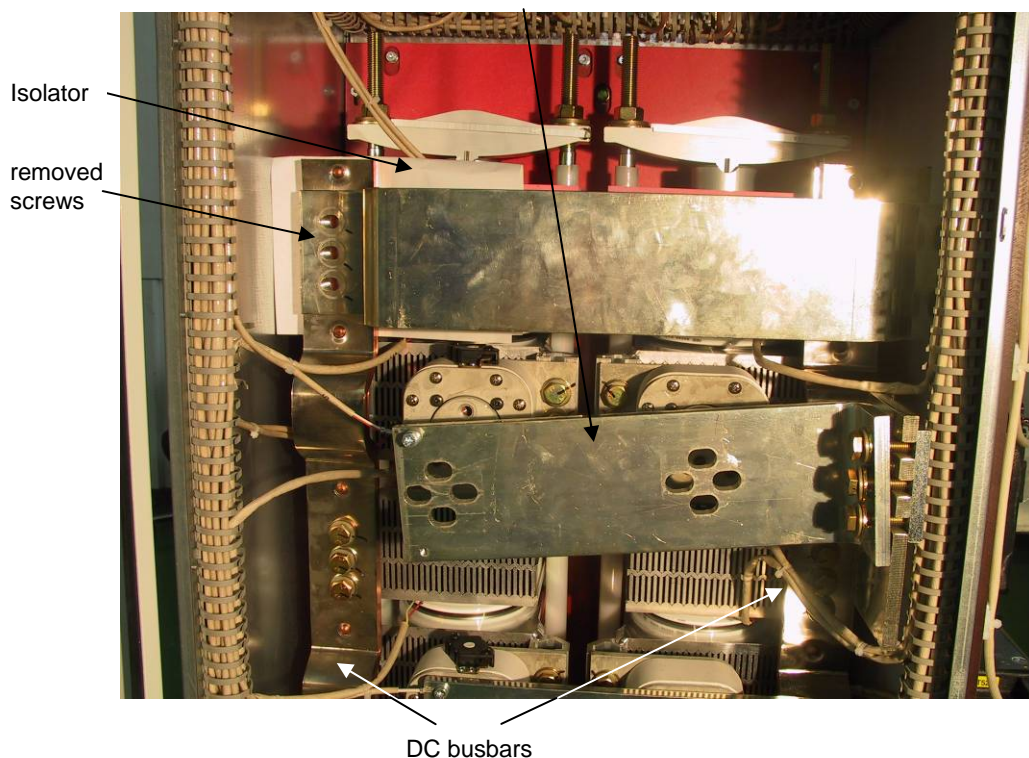
Location of busbars
