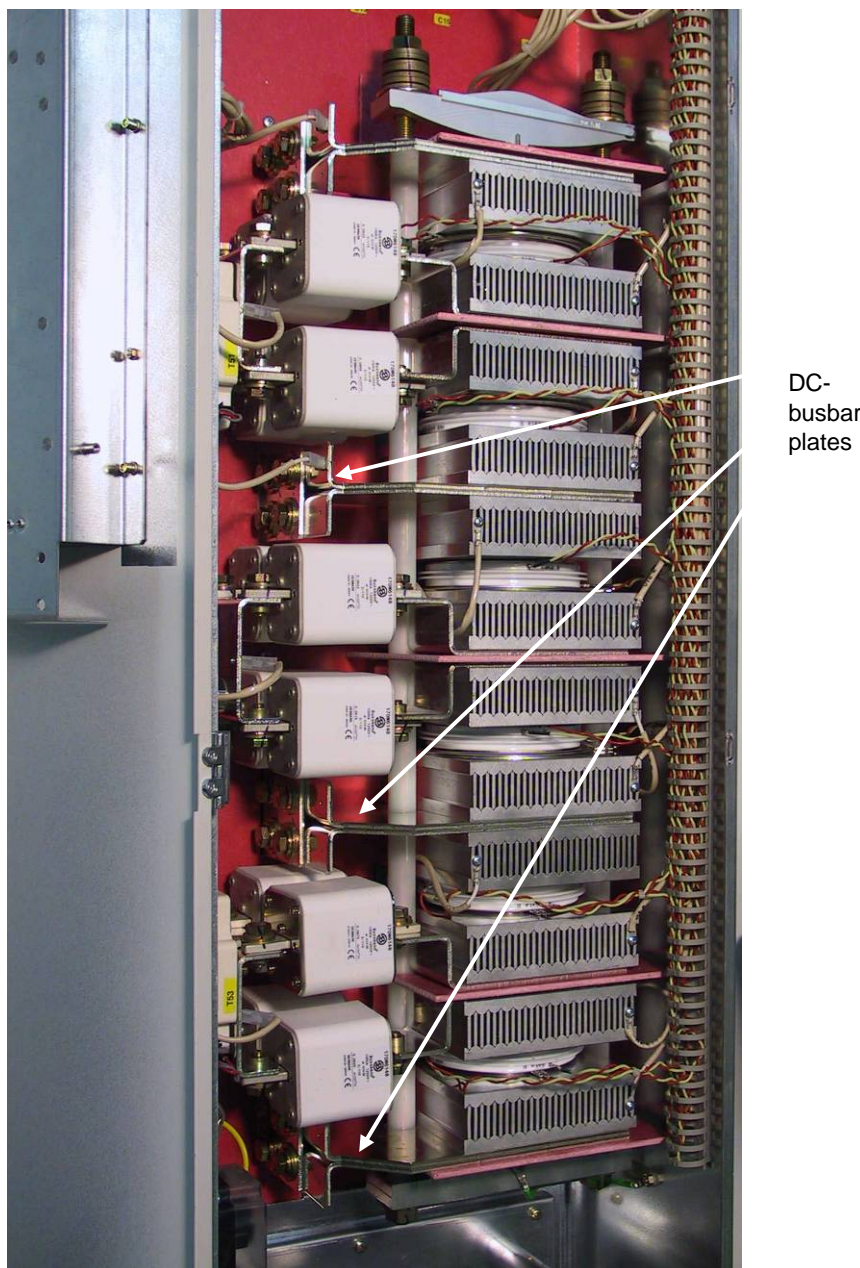
Location of the DC - busbar plates
