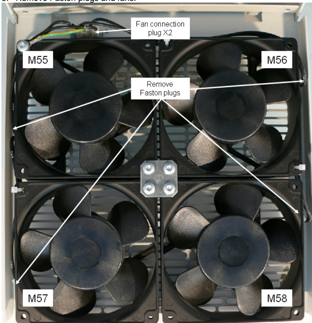
Faston plugs
