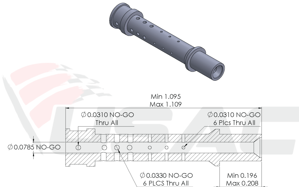
GX 160 UT1 MAIN NOZZLE
