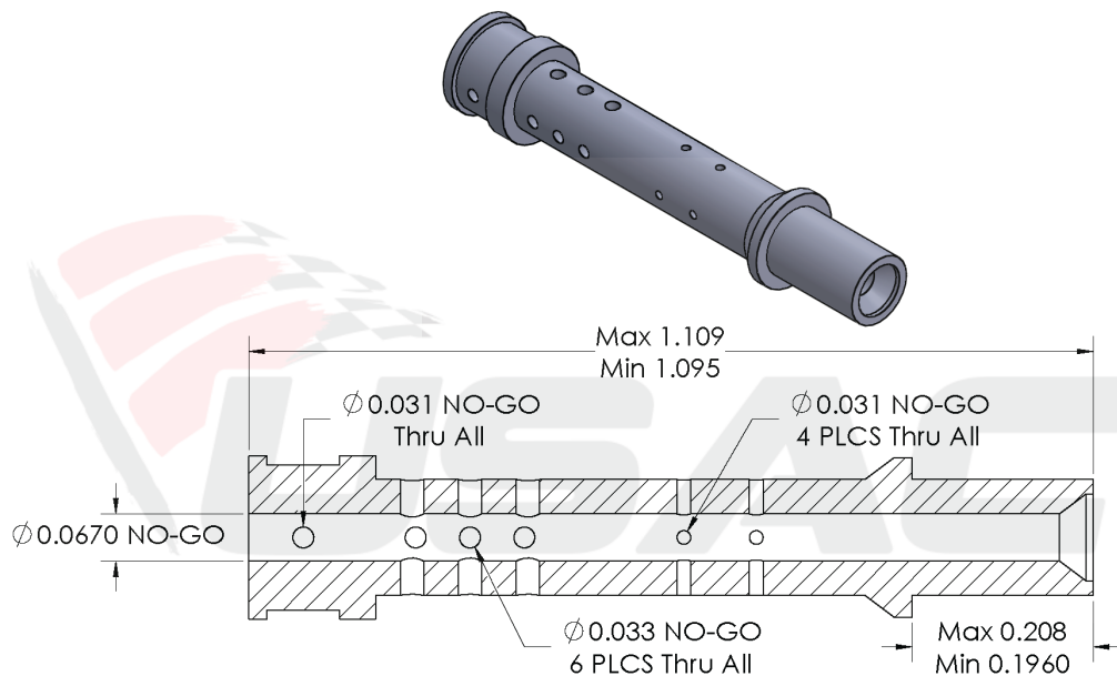
GX 200 MAIN NOZZLE
