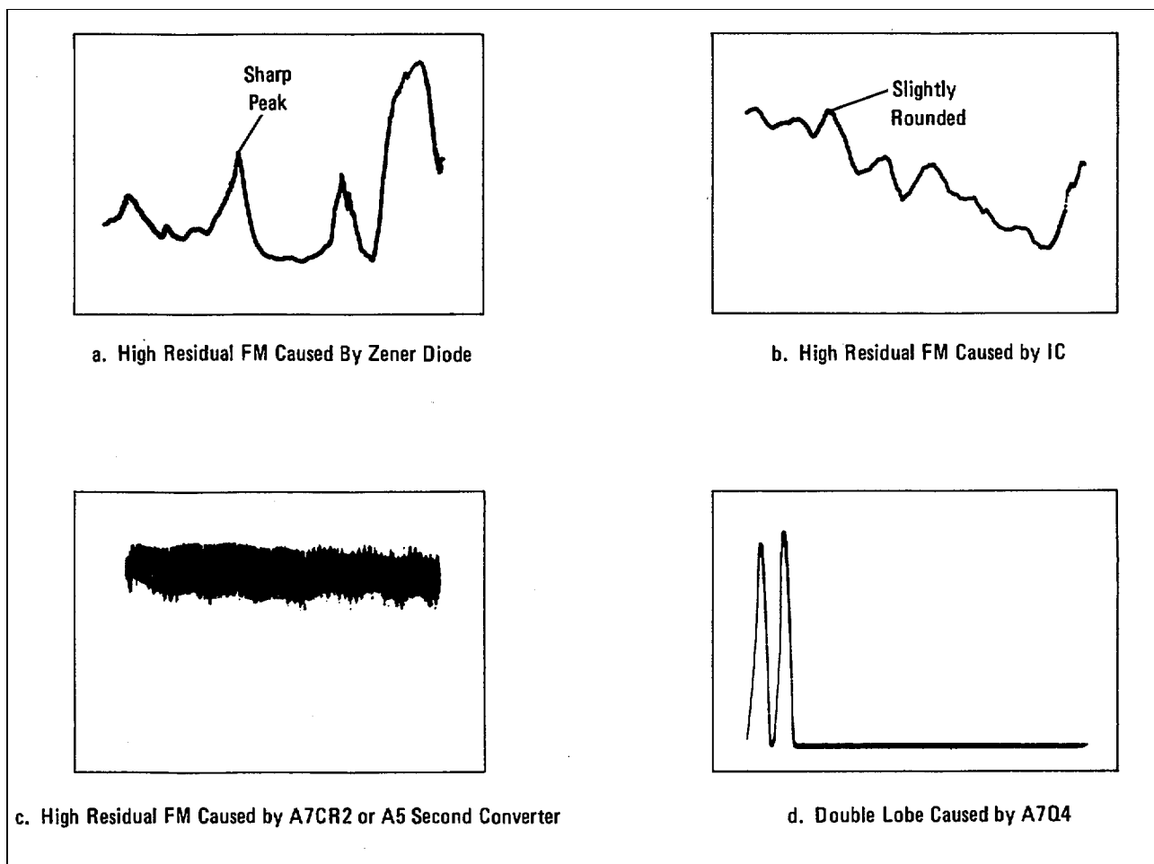
Figure 8-3. CRT Displays for Residual FM Troubleshooting
