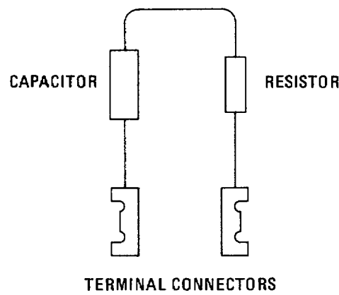
Figure 5-7. Crystal Short Configuration
