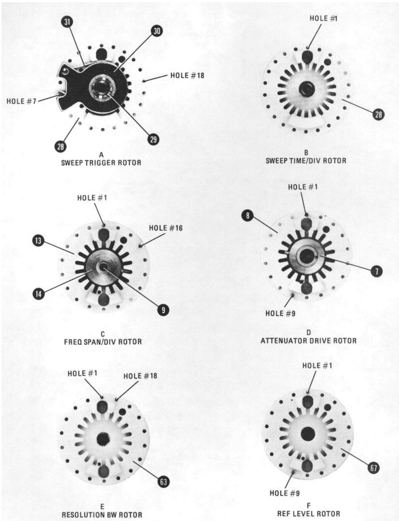
Figure 8-49. Rotor Assemblies
