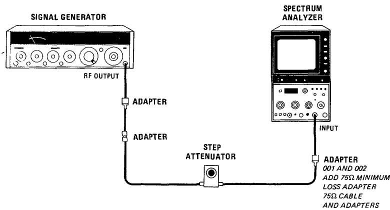
Figure 4-19. Reference Level Accuracy Test Setup
