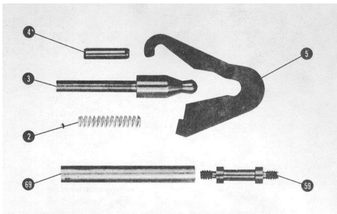
Figure 8-50. Machined Parts
