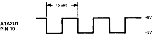
Figure 8-7. A1A2U1 Clock
