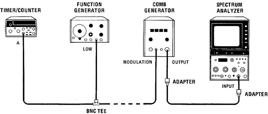
Figure 4-1. Frequency Span Accuracy Test Setup
