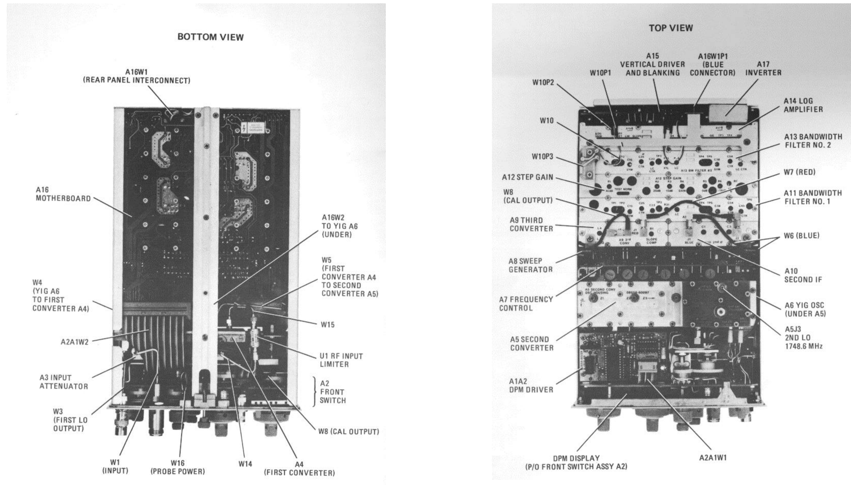
Figure 8-47. Location of Major Assemblies
