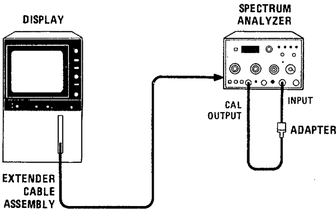
Figure 5-16. 1-dB Offset Adjustment Test Setup
