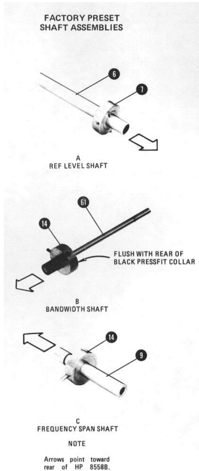
Figure 8-48. Shaft Assemblies
