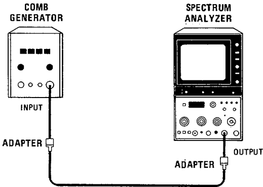
Figure 4-5. Residual FM Test Setup
