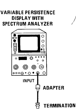
Figure 4-16. Residual Responses Test Setup
