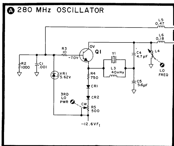
Figure 7-8. P/O A9 Third Converter and A10 Second IF Schematic Diagram (CHANGE C)
