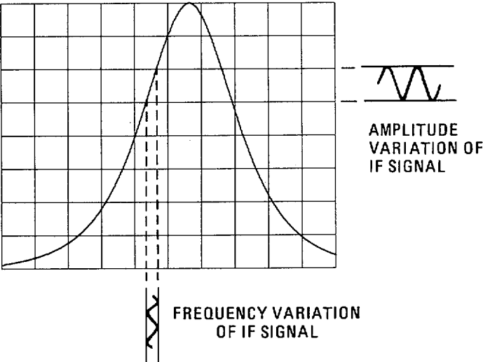
b. Shape of 10 kHz Resolution BW Filter
