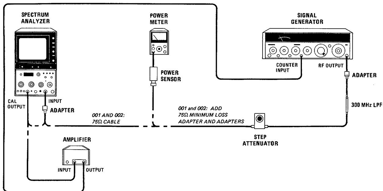
Figure 4-21. Calibrator Accuracy Test Setup
