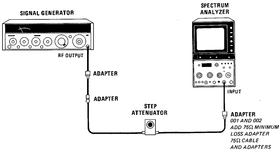
Figure 4-18. Input Attenuator Accuracy Test Setup
