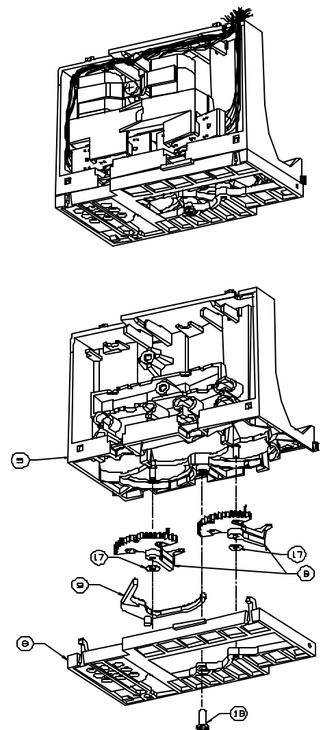
BACK VIEW
