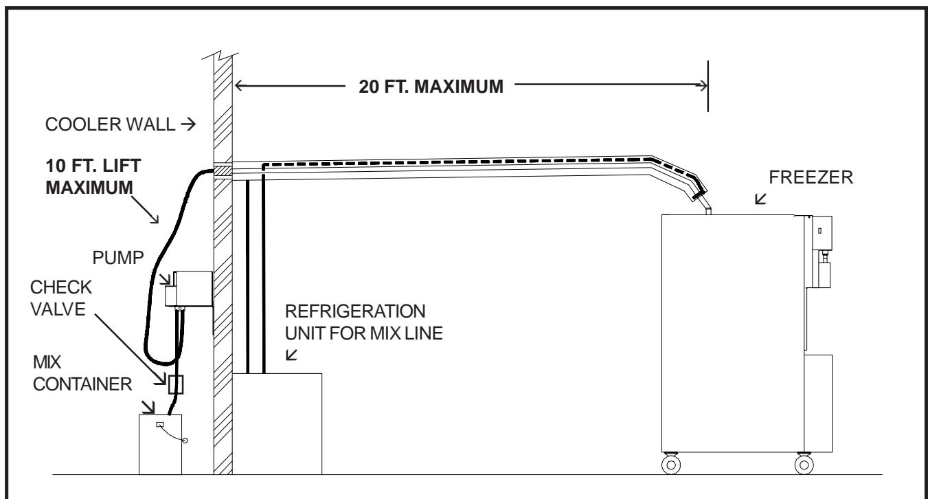
Figure 2 Mix Transfer Line
