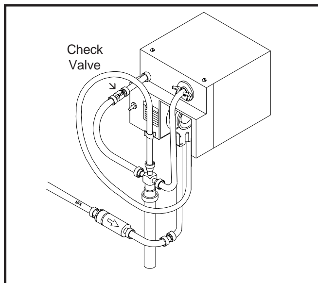
Figure 6 Removing Parts
