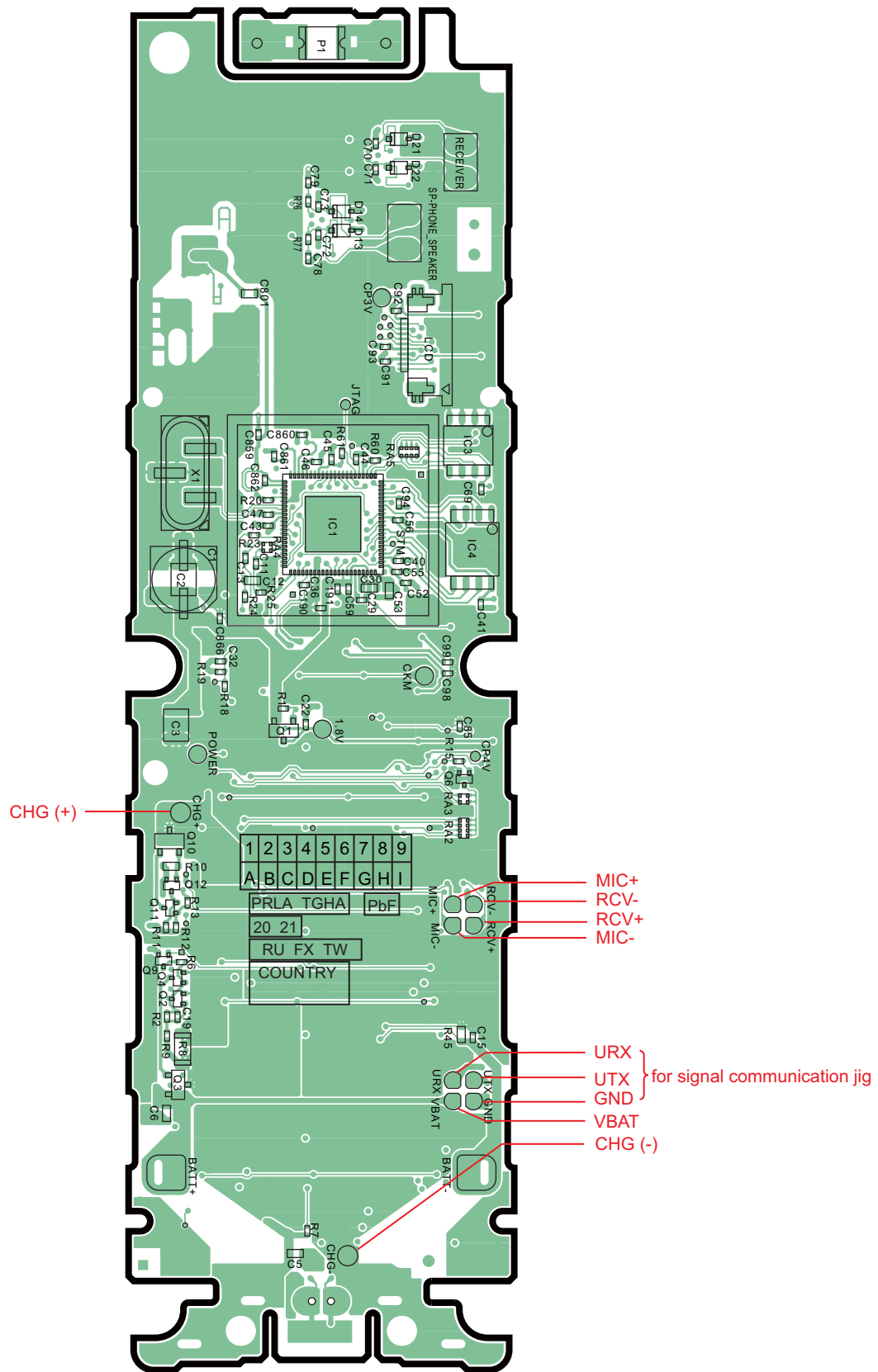
KX-PRLA20 CIRCUIT BOARD (Handset_Main (Component View))
