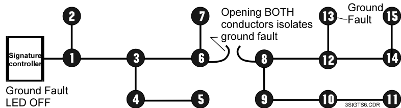
Figure 8-10: Ground fault isolation
