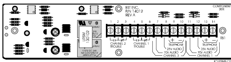
Figure 4-5: URSM
