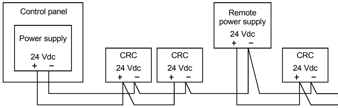
Figure 3-17: Wiring for remote power supply
