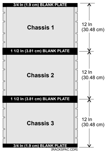
Figure 5-6: Rack-mounted chassis
