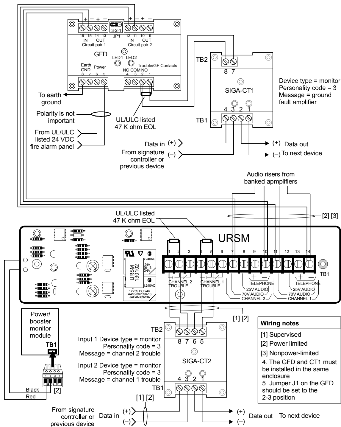
Figure 4-6: URSM wiring
