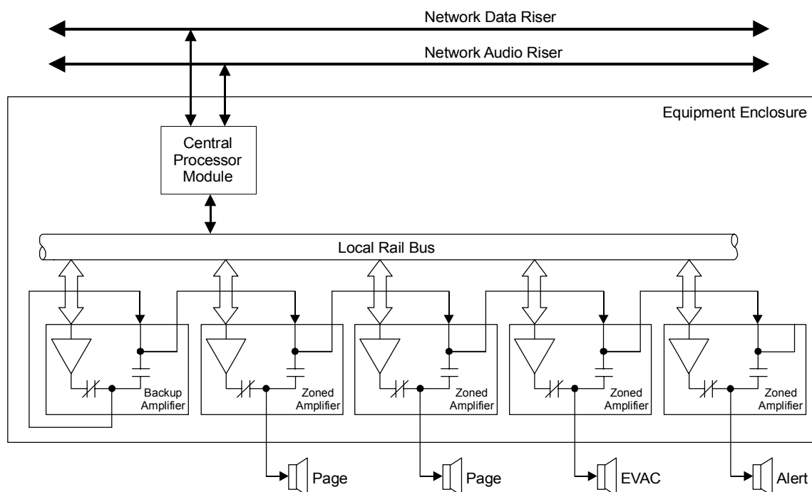
Figure 1-4: Normal amplifier operation
