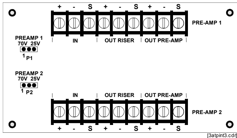
Figure 4-3: 3-ATPINT Interface Card
