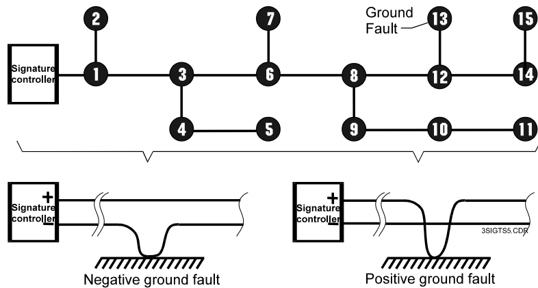
Figure 8-9: Signature data circuit ground faults
