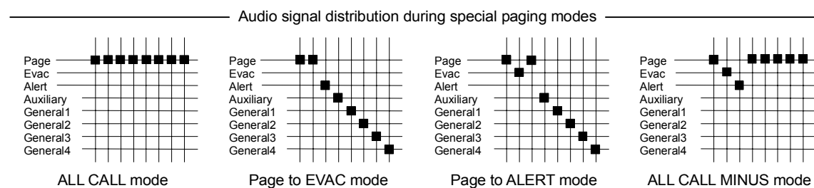
Figure 1-8: Audio Source Unit Special Page Mode Signal Flow
