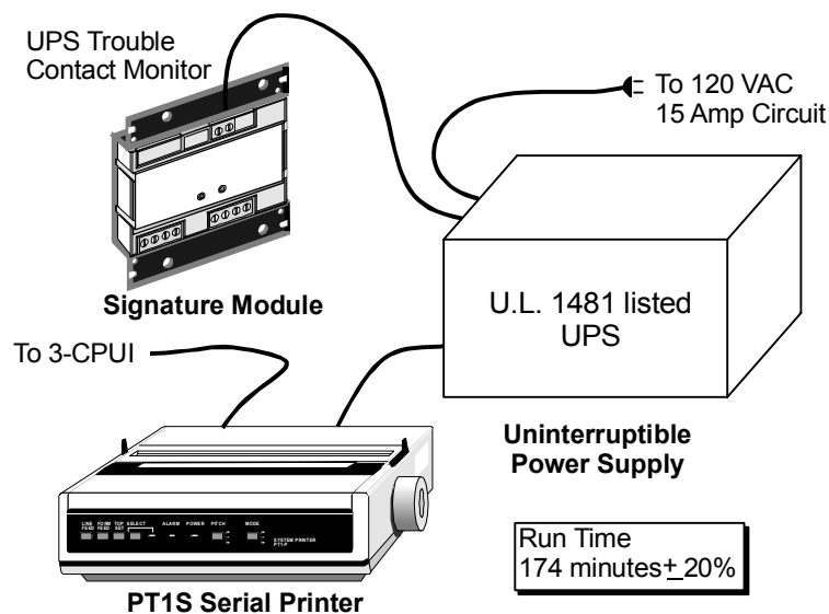
Figure 5-10: Printer uninterruptible power supply wiring
