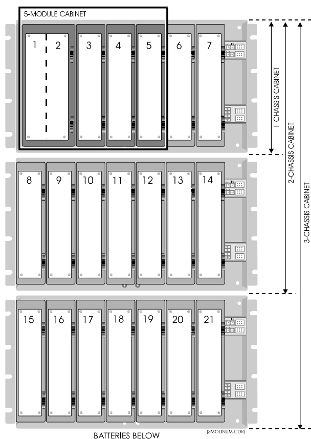
Figure 5-7: Local rail module slot identification
