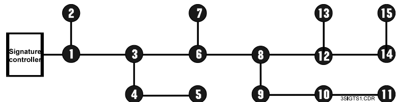
Figure 8-5: Normal circuit topology
