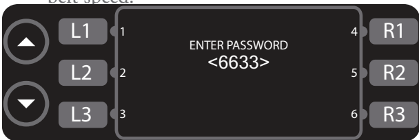
Figure 15: Password Screen
