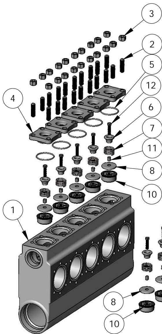
Q5450C-33C-A FLUID END ASSEMBLY
