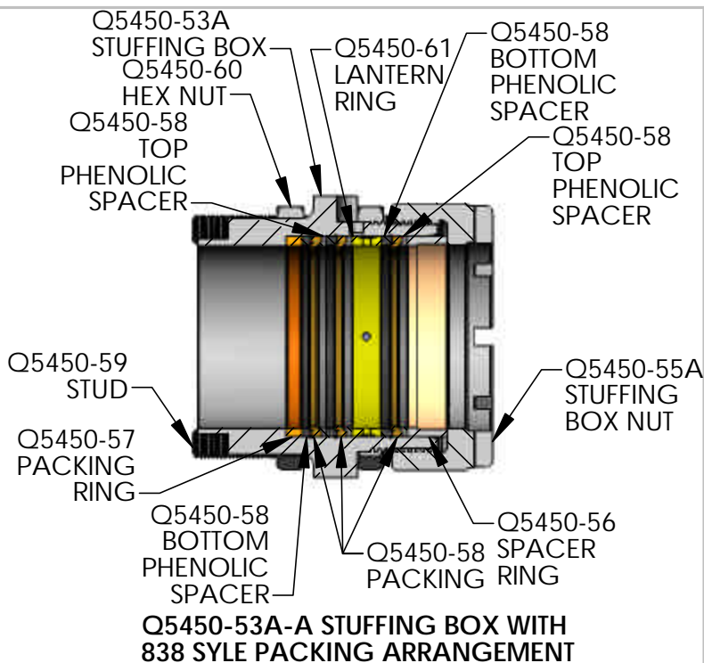
Q5450C PARTS ILLUSTRATION
