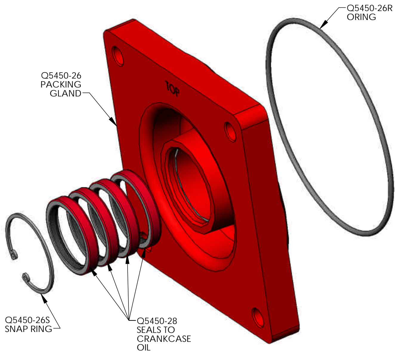
Q5450-26-A PONY ROD PACKING GLAND ASSEMBLY
