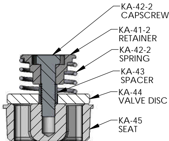
KA-39-2-A DISC VALVE ASSEMBLY
