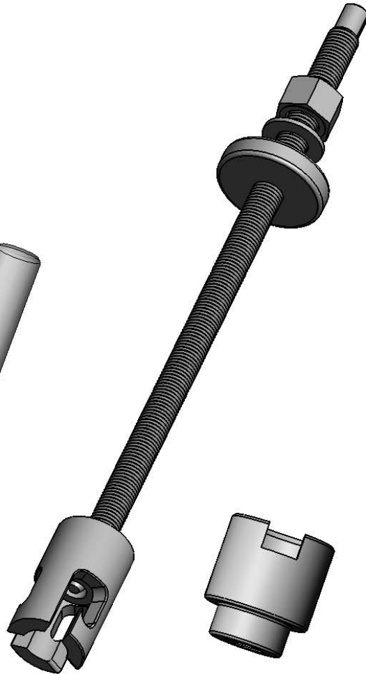
KA-555 DISC SEAT "J" TYPE PULLER ASS'Y
