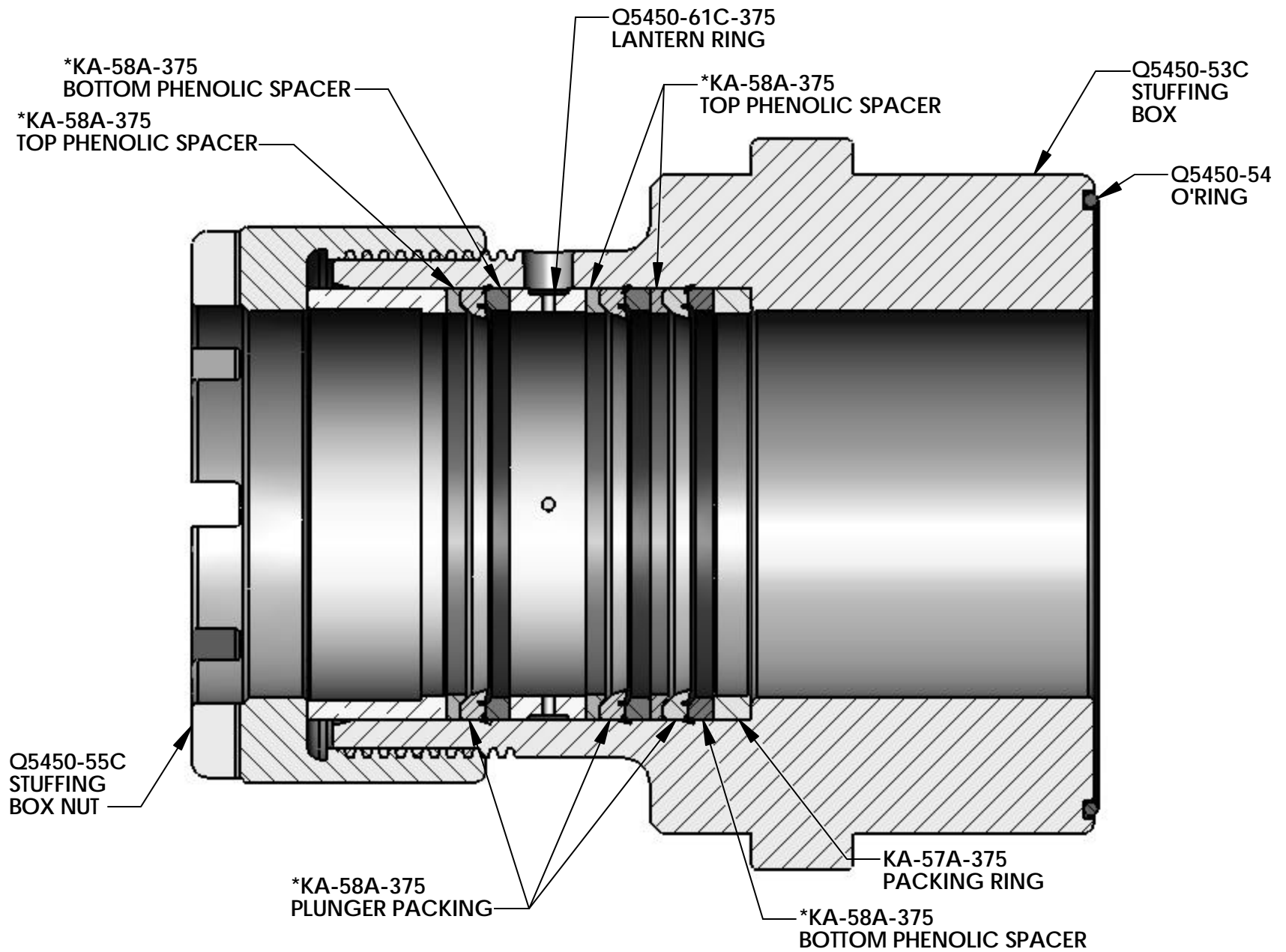
Q5450 "C" BOX "J" STYLE PACKING ARRANGEMENT (FOR 3.750" PLUNGERS)
