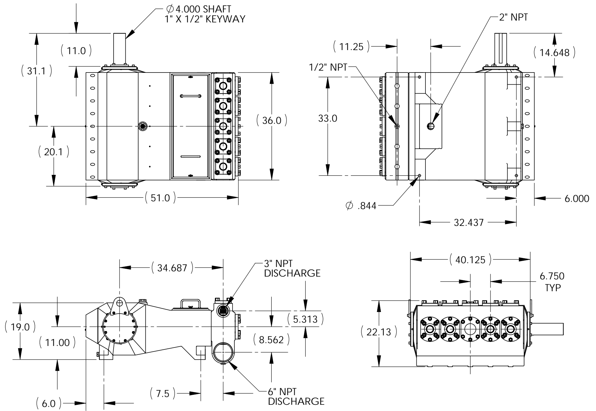
Q5450C GENERAL DIMENSIONS
