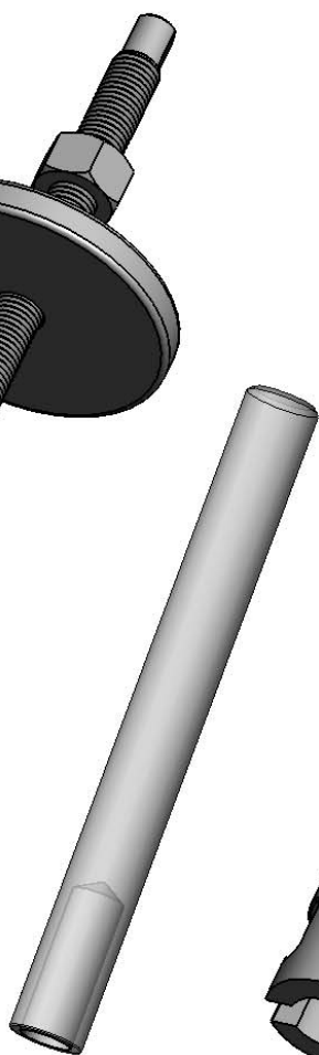
KA-306 VALVE SEAT SEATING TOOL
