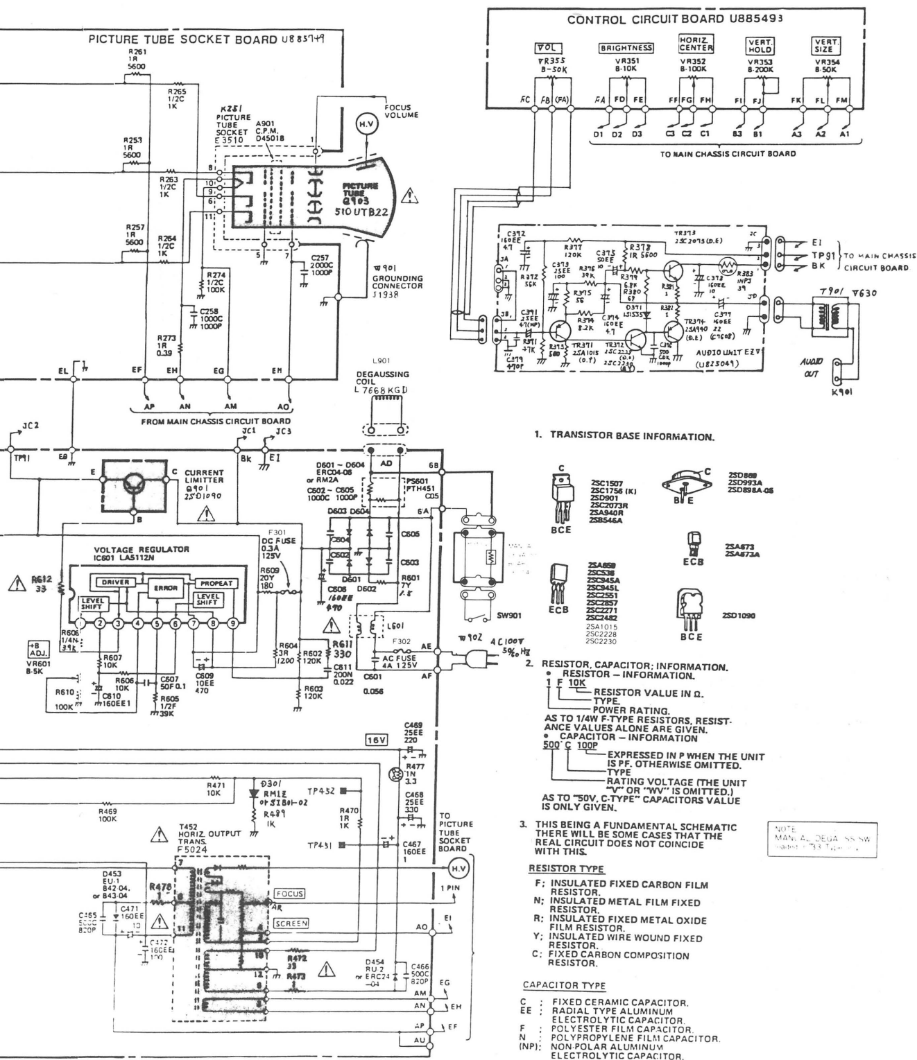
Figure 7 Sanyo Model 20-EZV Video Display Schematic Diagram, Sheet 1
