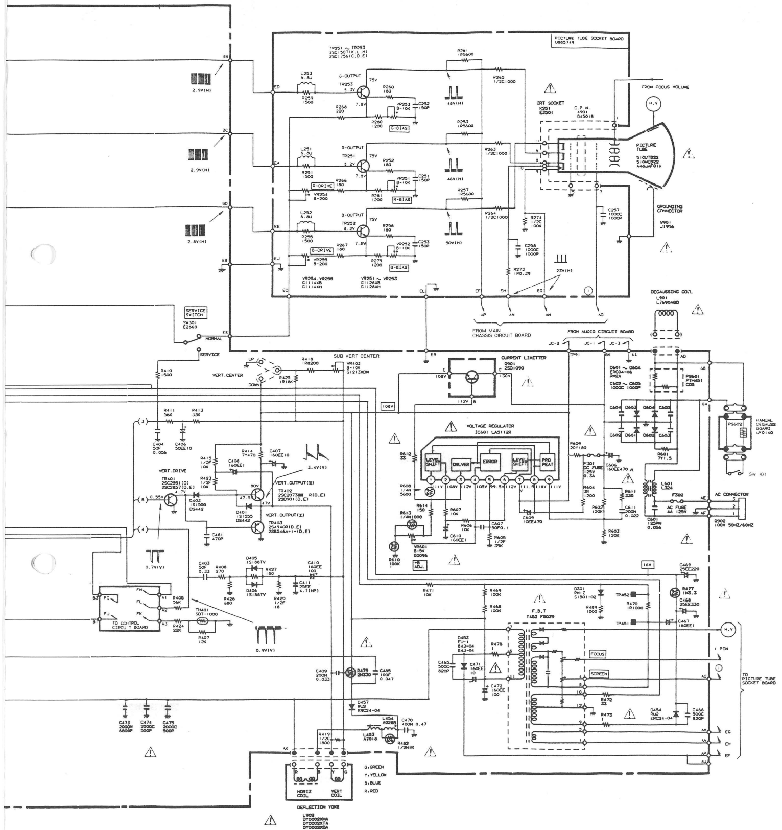
Figure 8 Sanyo Model 20-Z2AW Video Display Schematic Diagram
