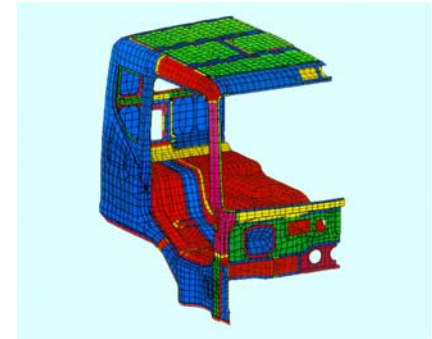
Computerized Cab Design
