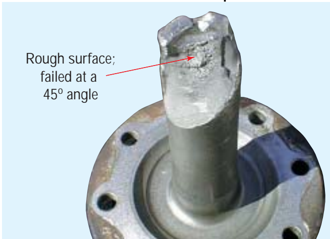
Torsional Shock Failure - Close up
