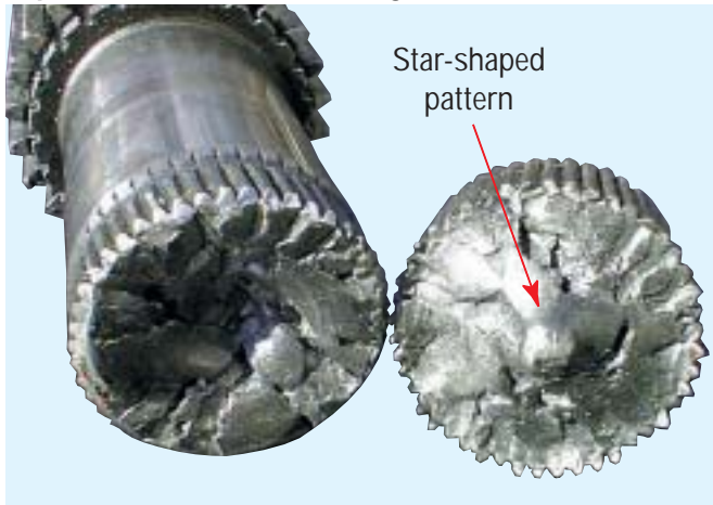
Output Shaft - Torsional Fatigue Failure
