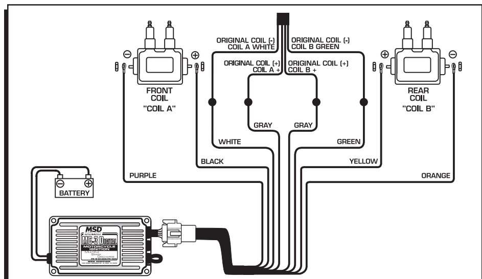
Figure 4 Wiring to a Stock Dual Coil Ignition System.
