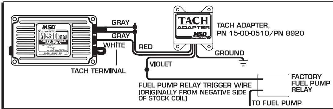
Figure 7 Installing a Tach Adapter.
