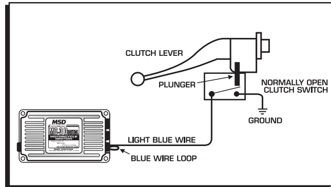
Figure 10 Wiring the Two Step Module Selector.
