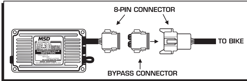
Figure 11 Bypassing the MSD MC3.
