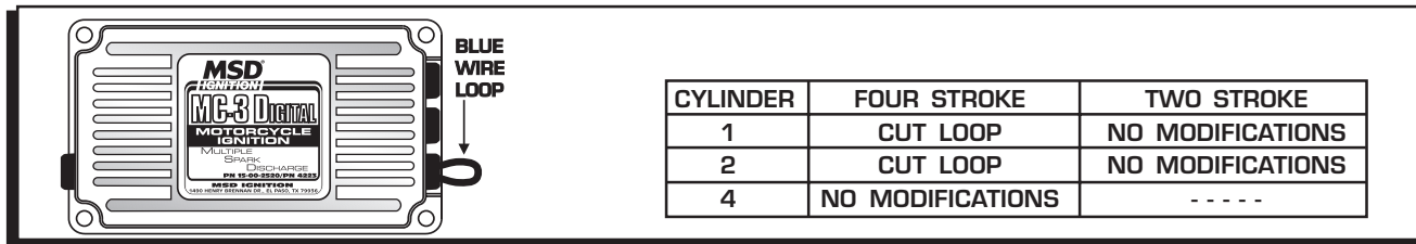
Figure 1 Cylinder Select Wire Loop.
