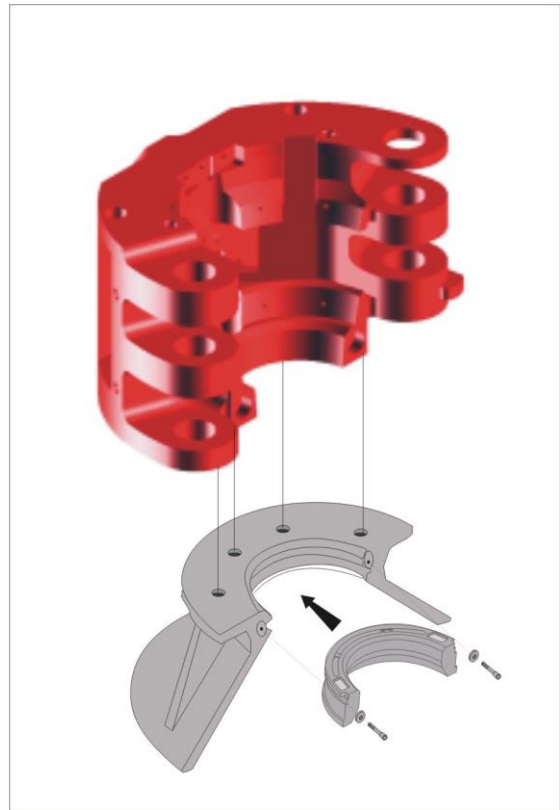
Figure 2-4. Elevator Guides
