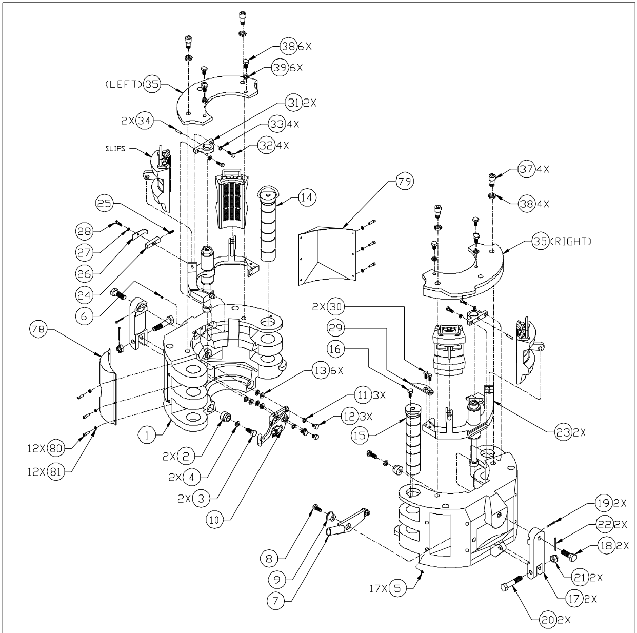
Figure 8-4. 200/250 Ton Air Operating Elevator/Spider Assembly (Part 1 of 3)
