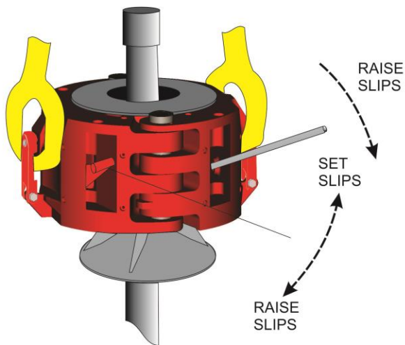
Figure 3-1. Operating Detail
