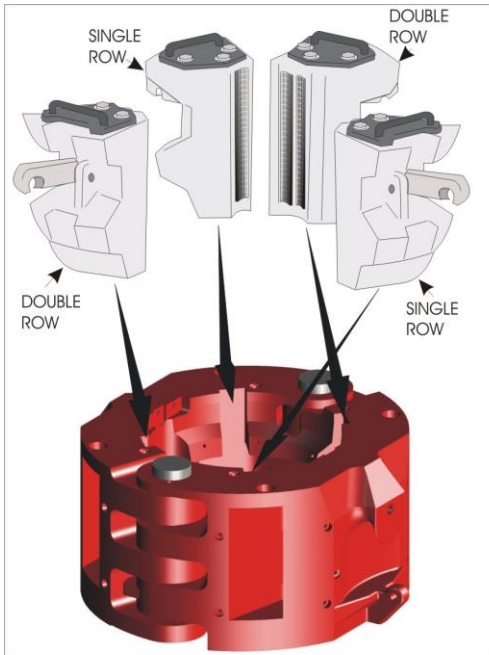
Figure 2-3. Double/Single Inserts
