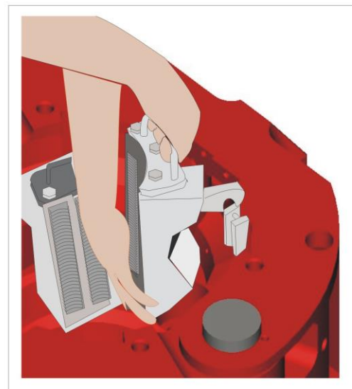
Figure 2-2. Slip Detail
