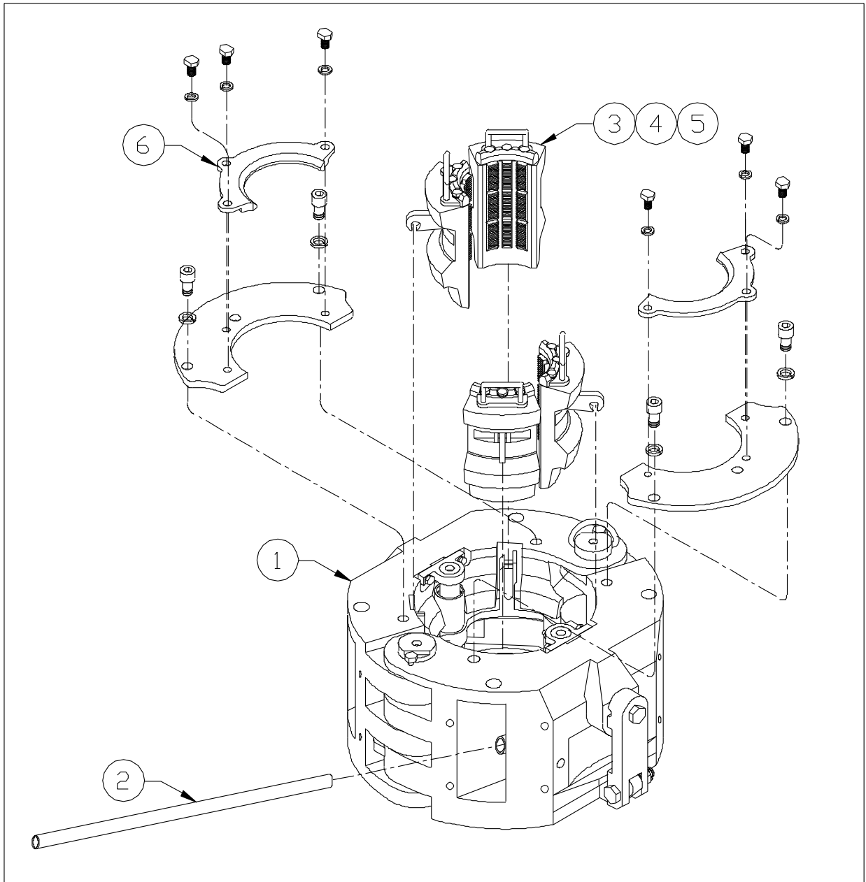
Figure 7-2. 200/250 Ton Spider Assembly
