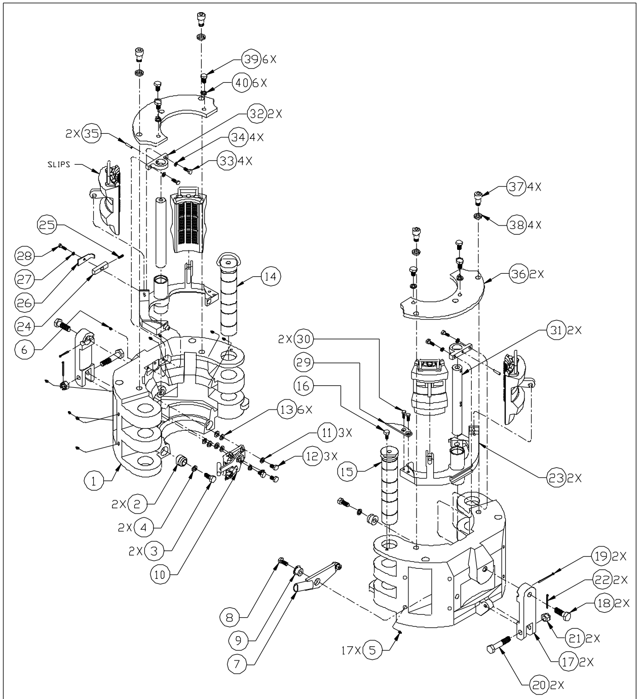
Figure 7-4. 200/250 Ton Elevator/Spider Assembly
