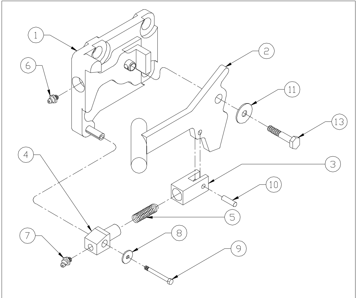
Figure 7-6. Latch Assembly
