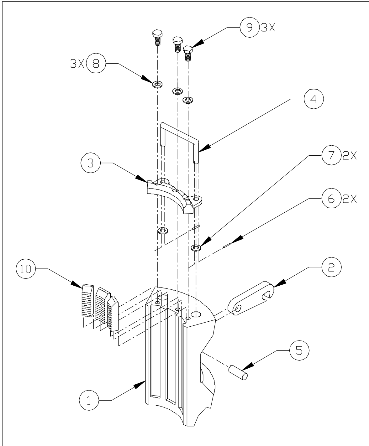
Figure 7-8. Multi-Insert Slips
