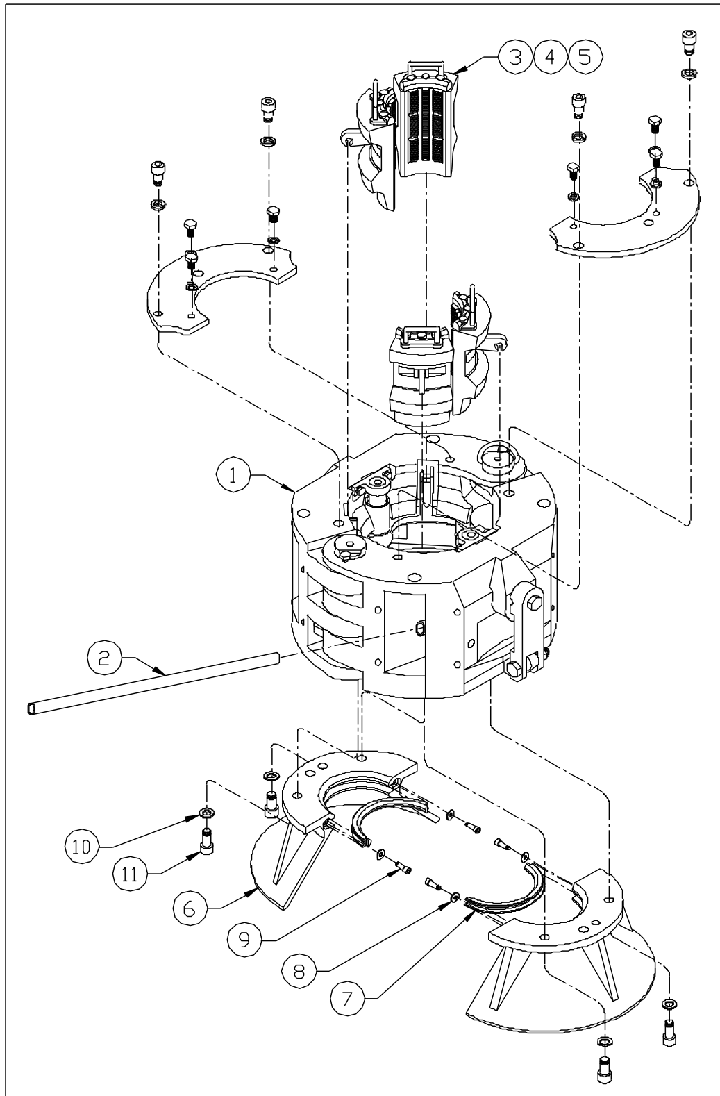
Figure 7-3. 200/250 Ton Elevator Assembly
