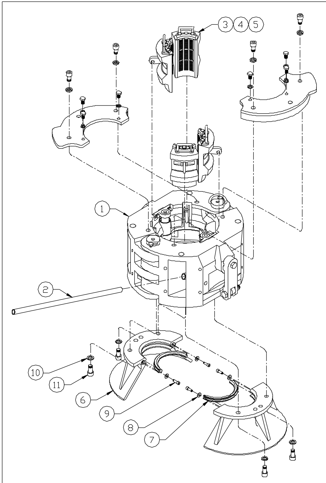
Figure 8-3. 200/250 Ton Air Operating Elevator Assembly
