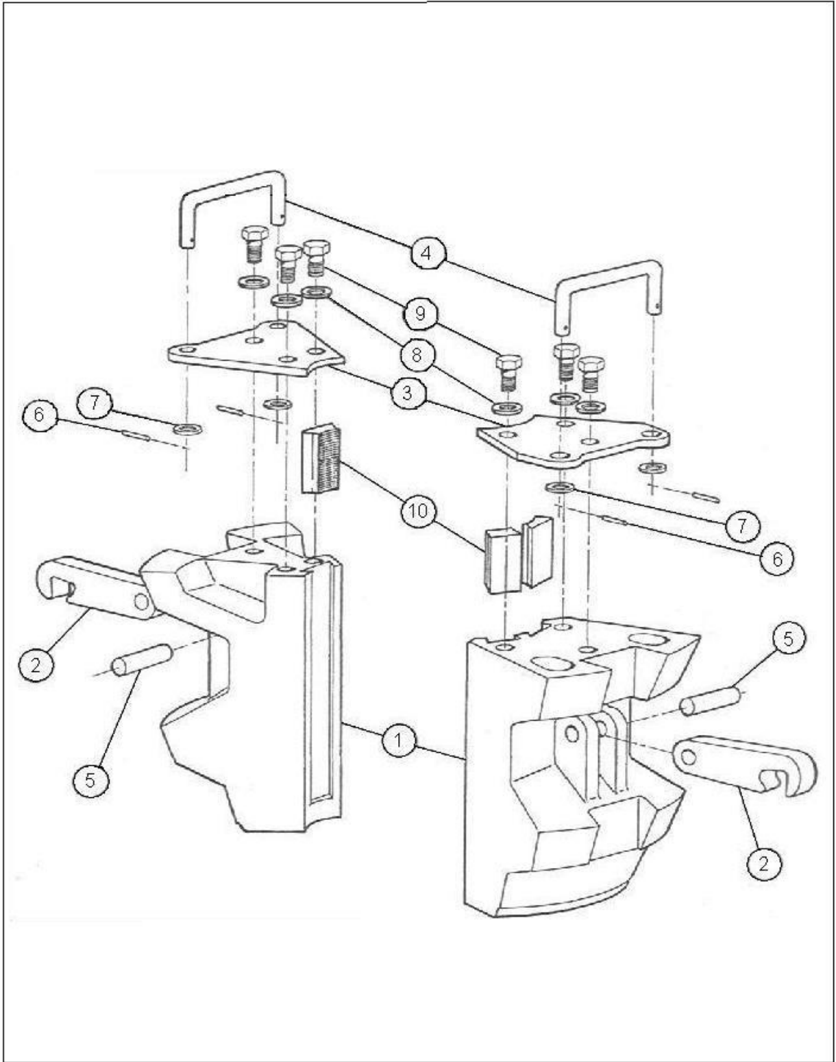
Figure 7-9. Double/Single Insert Slips
