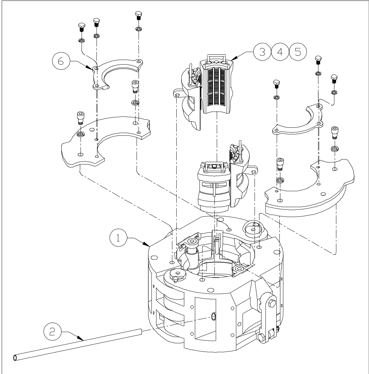
Figure 8-2. 200/250 Ton Air Operating Spider Assembly
