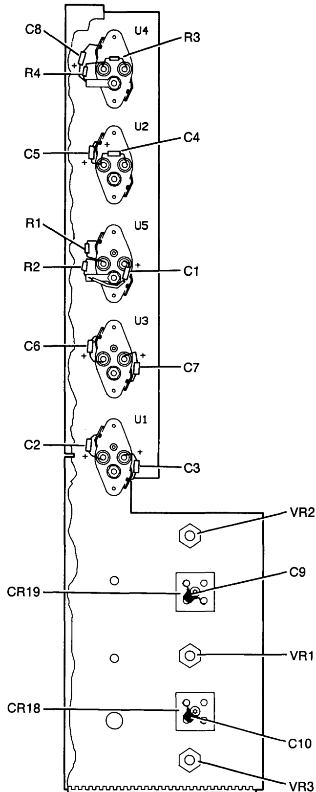
Figure 11. Parts Identification (Regulator Assembly)
