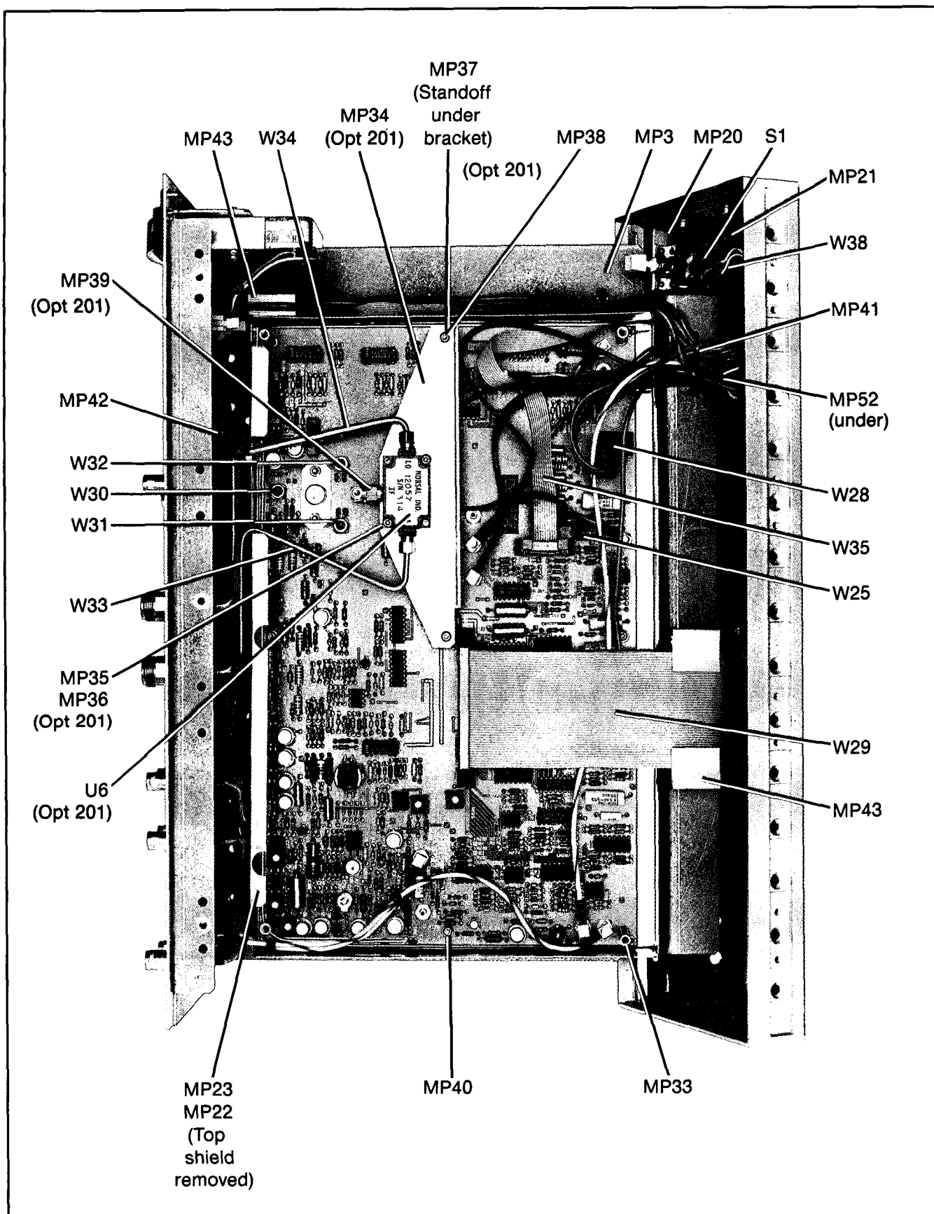
Figure 9. Parts and Cable Identification (Top View)
