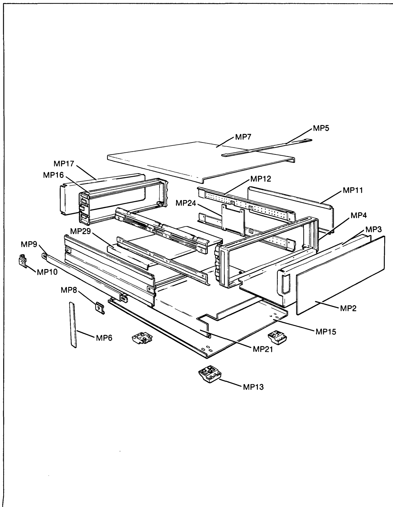
Figure 6. Cabinet Parts
