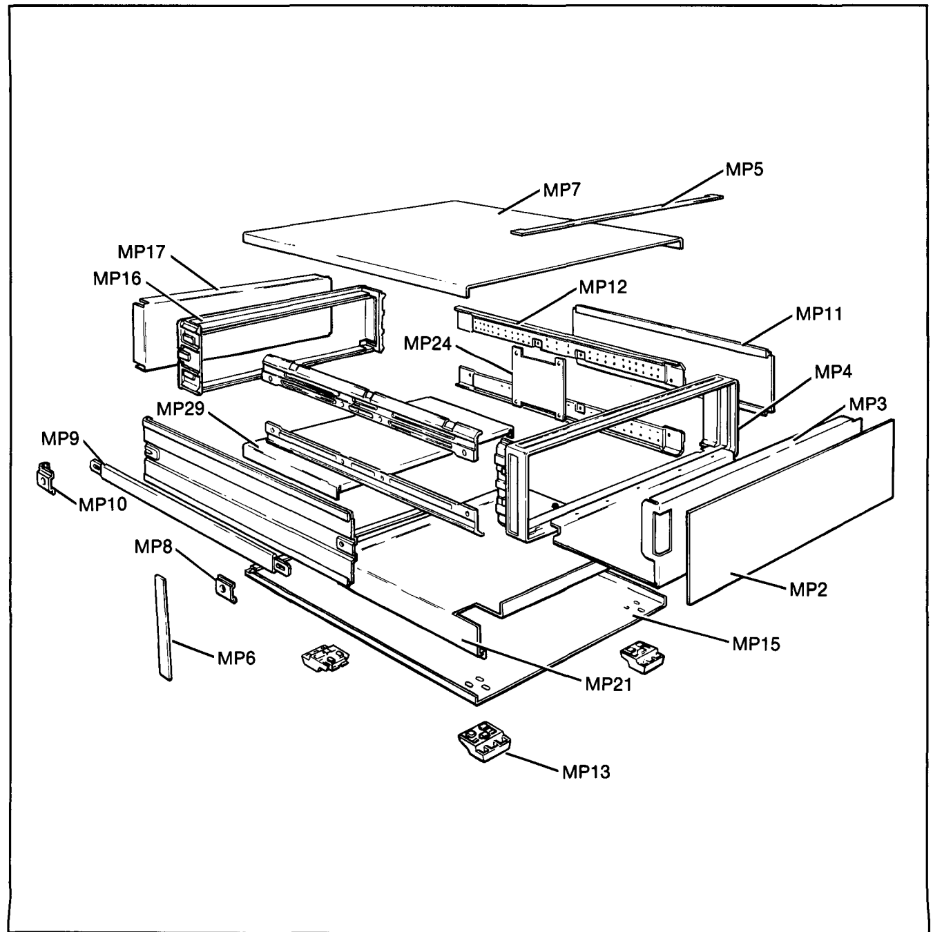
Figure 6. Cabinet Parts
