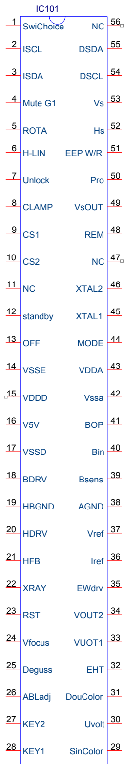
IC101 SAA4849P
