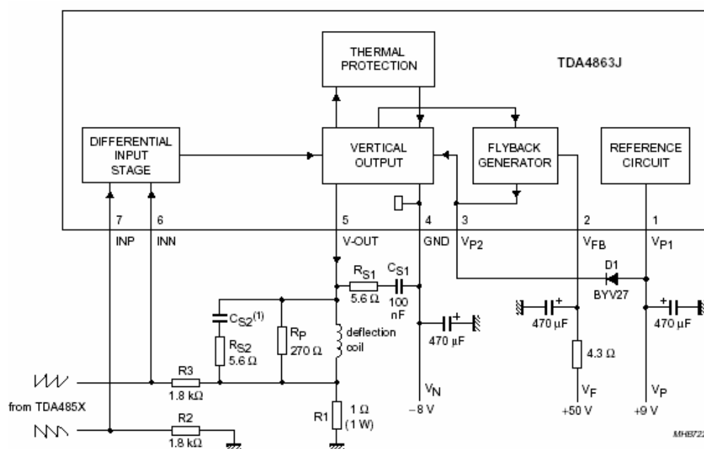
IC601 TDA4863A
