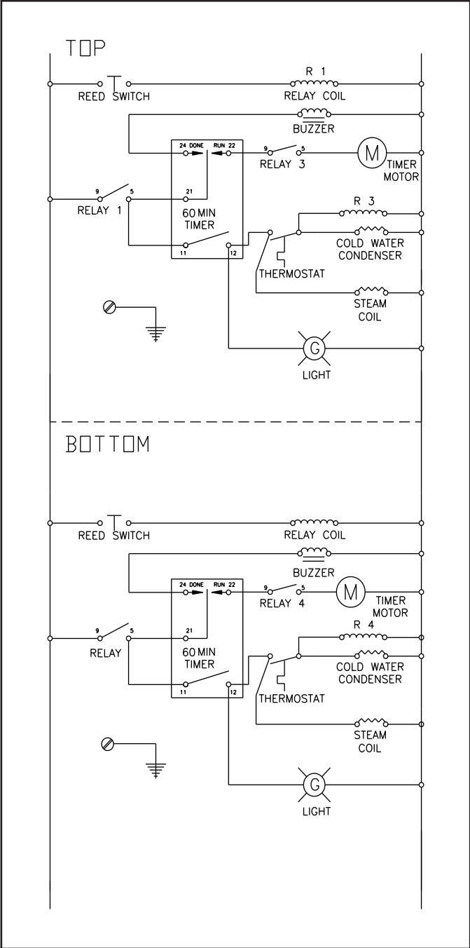
WIRING SCHEMATIC FOR STEAMER
