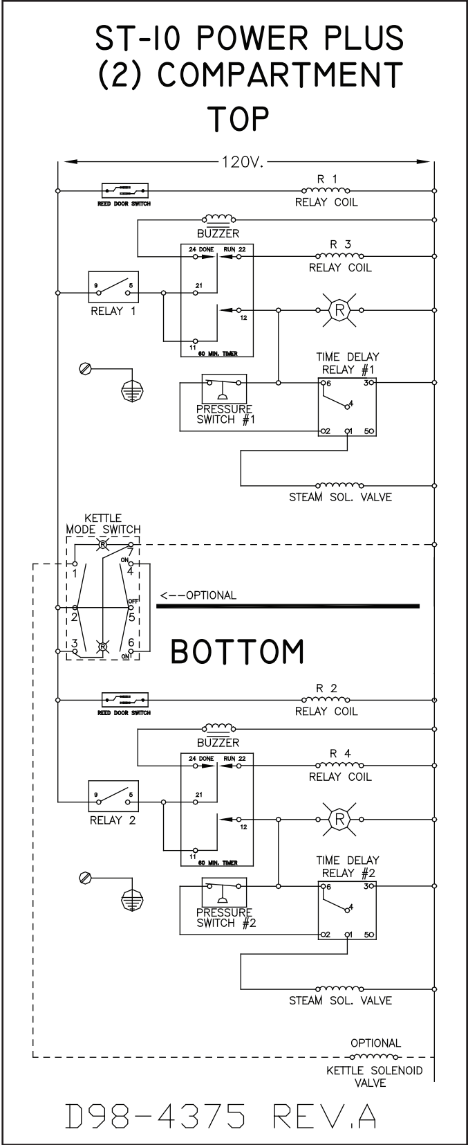
WIRING SCHEMATIC FOR POWER PLUS
