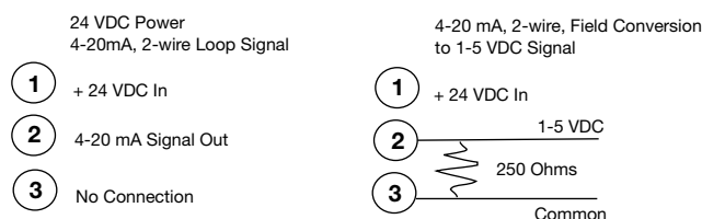
Wiring Connections
