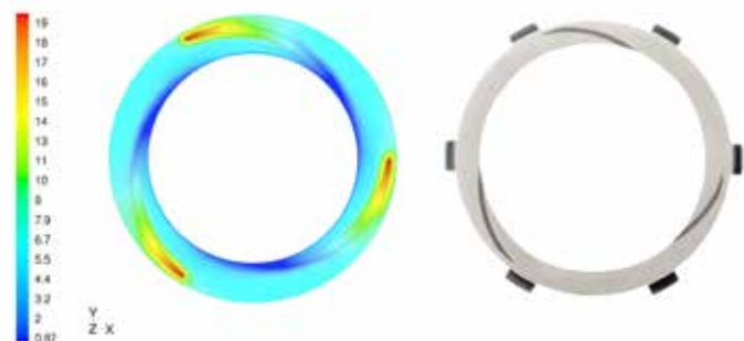
Pressure distribution in grooved seal face.
