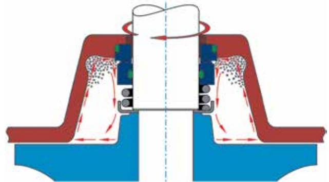
Wear in traditional seal cavity
