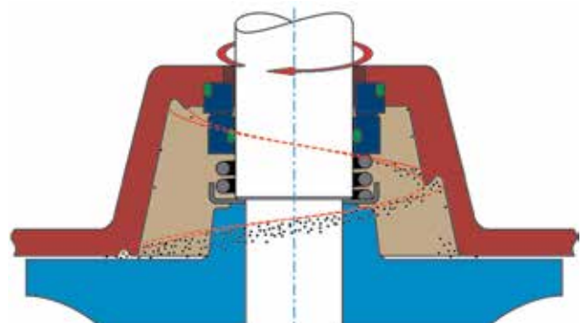
Particles expelled by Spin-out seal cavity
