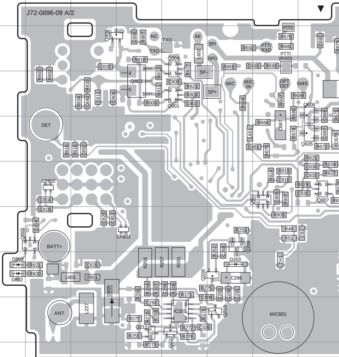
TX-RX UNIT (X57-6730-10) Component side view (J72-0896-09)
