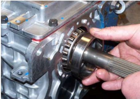
FIG. D (TKO ONLY) INSTALL BEARING RACE IN TRANS
