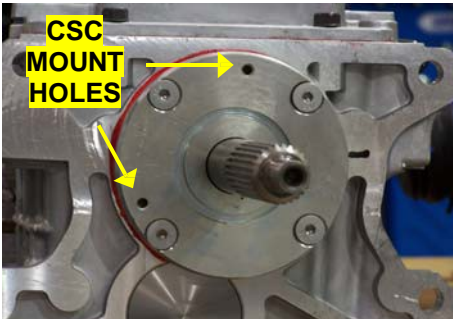
FIG. G RETAINER PROPERLY INSTALLED
