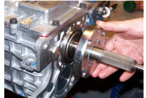
FIG. F INSTALL NEW RETAINER
