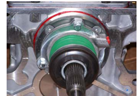
FIG. J CSC PROPERLY INSTALLED
