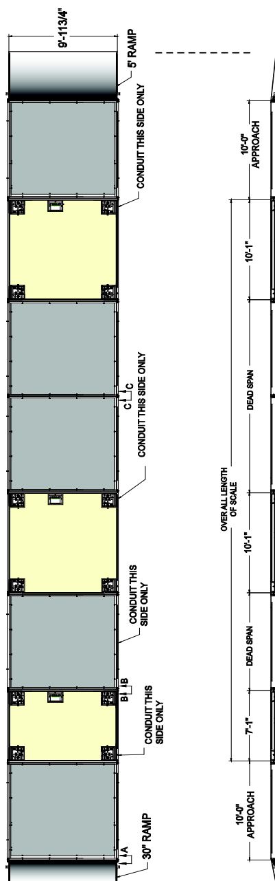
ELEVATION VIEW
