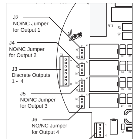
Figure 4-14: Optional Outputs & Jumpers
