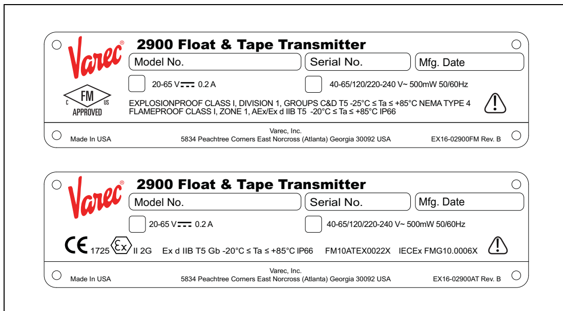
Figure 12-2: 2900 FTT Nameplate
