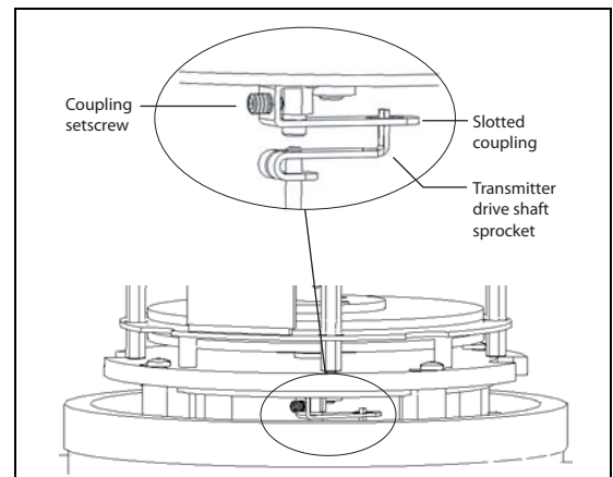
Figure 3-2: Transmitter Coupling
