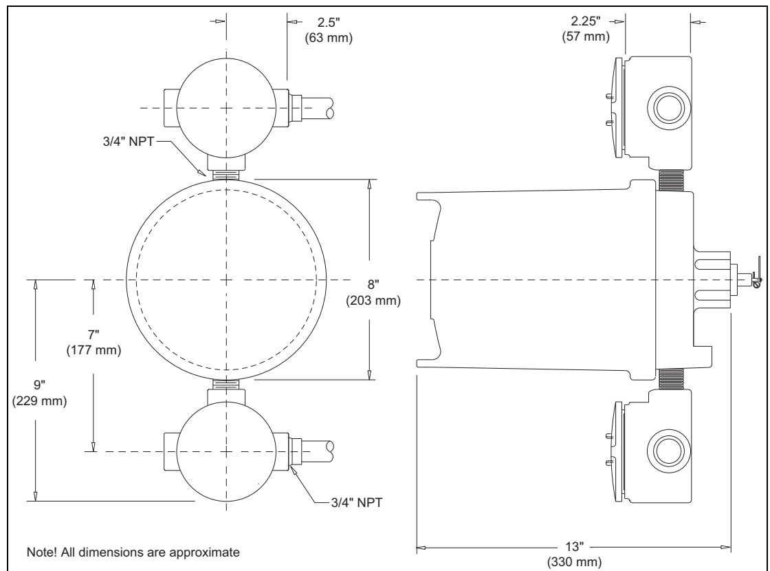
Figure 2-1: 2900 FTT Dimensions
