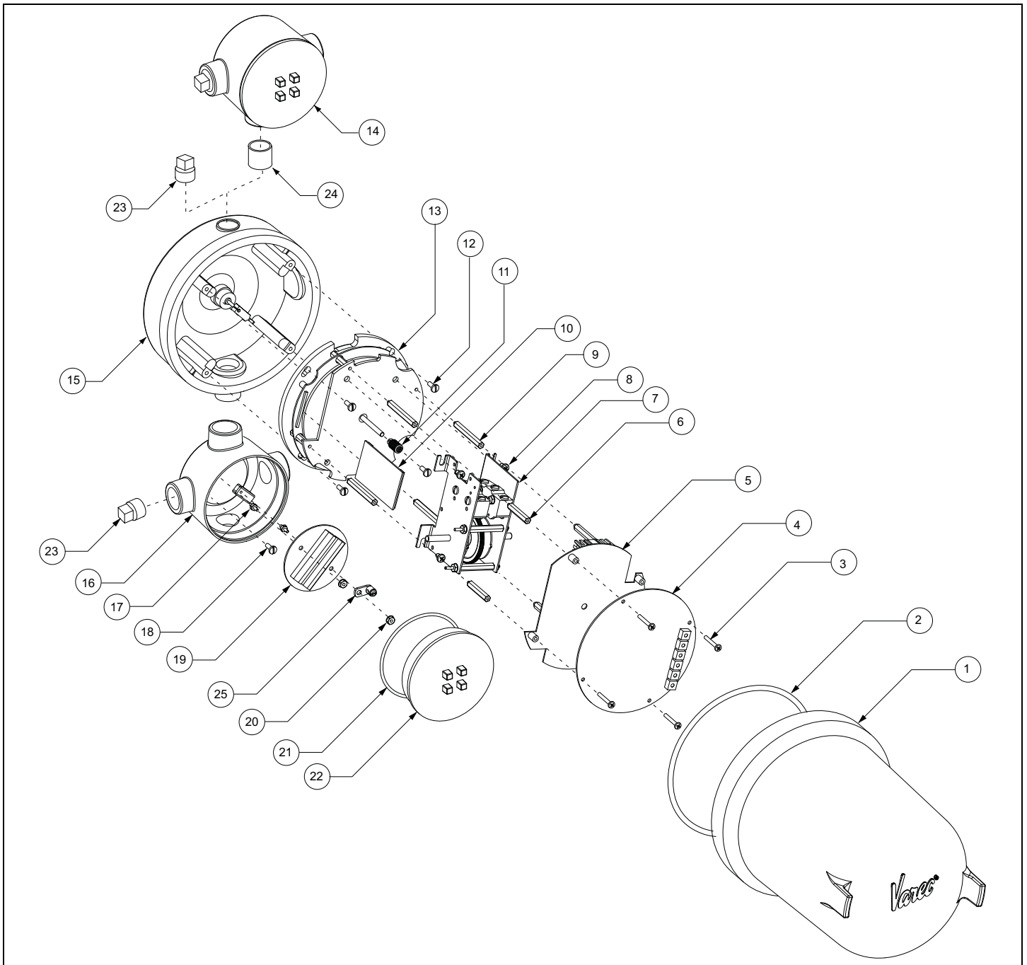
Figure 9-7: 2900 FTT Exploded Parts Diagram
