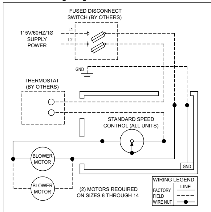
Standard Wiring Diagram for Cabinet Unit Heaters
