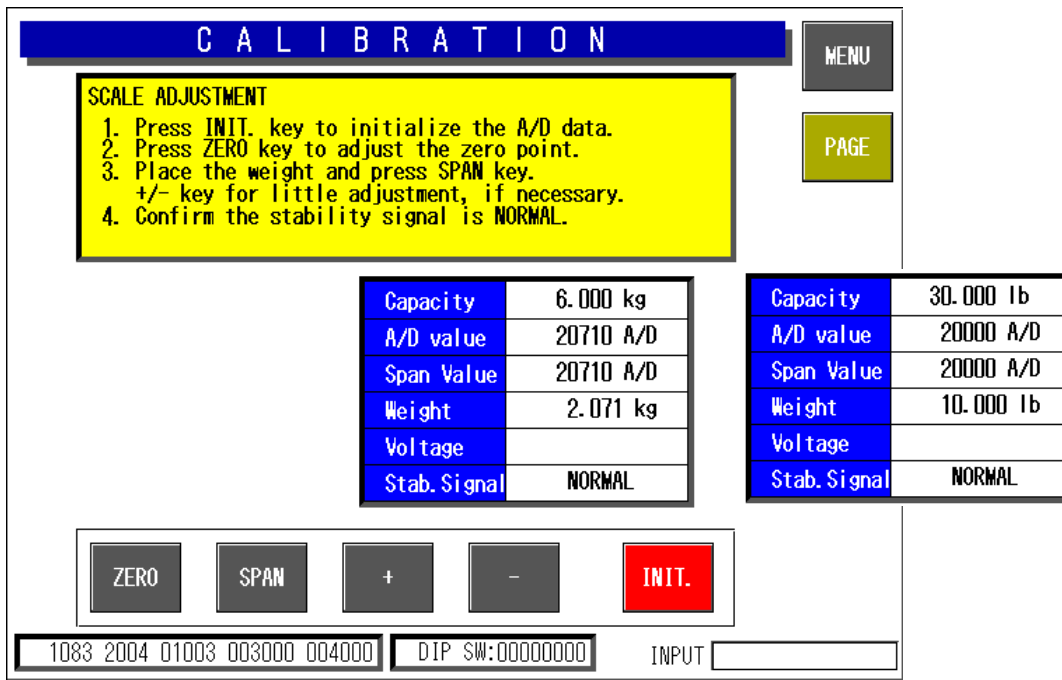
Calibration Screen
