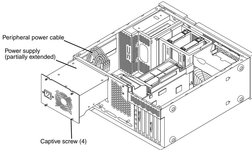
FIGURE 1-1 Removing the Power Supply
