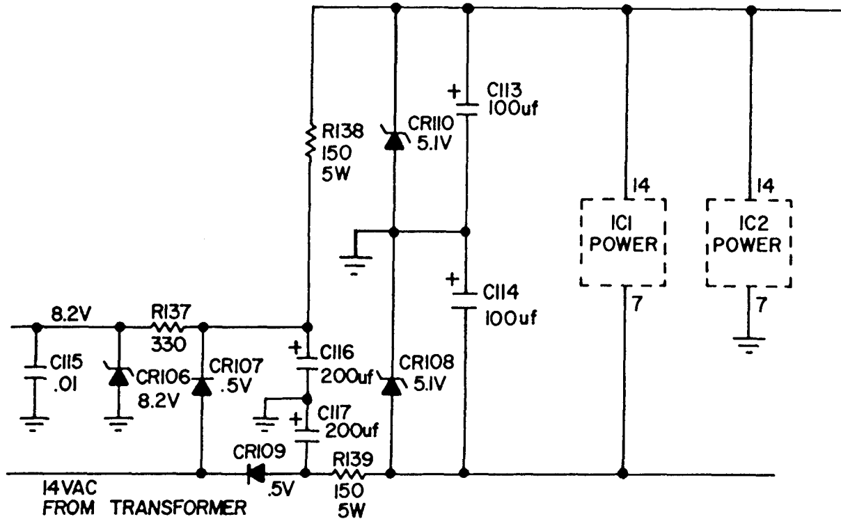
Fig. 9 Power Supply Schematic
