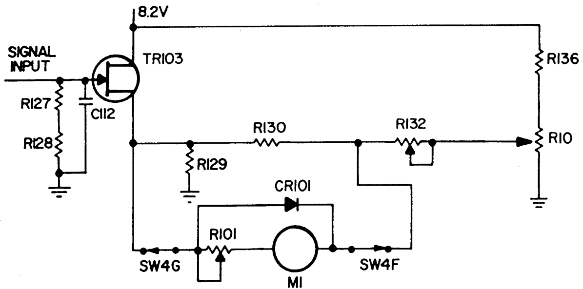
Fig. 6 Tube-test Bridge Circuit
