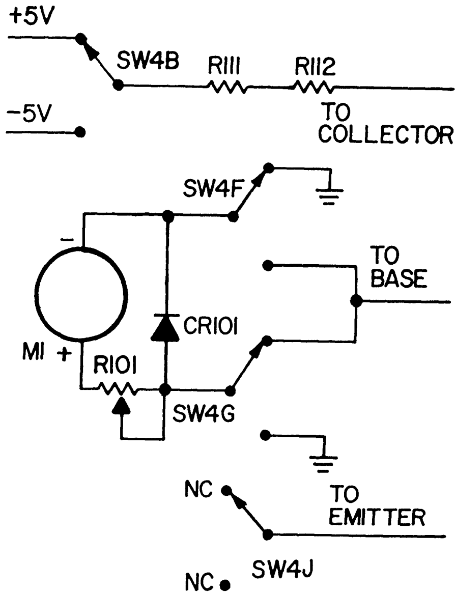
Fig. 12 Leakage Test Circuit
