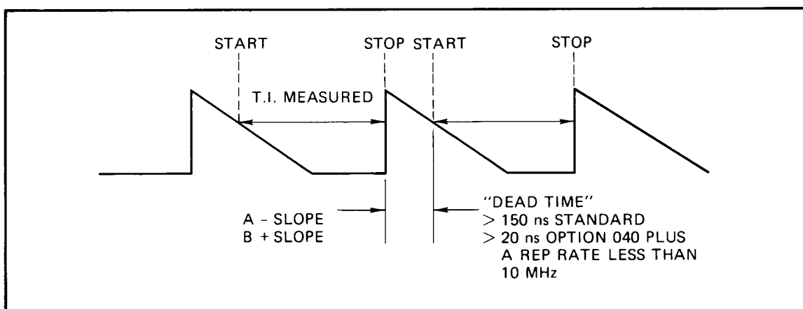
Figure 4-3. Dead Time
