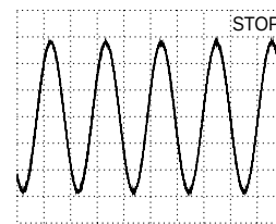
AC, 200mV/Div, 500μs/Div IC7400-(8)/-(9)
