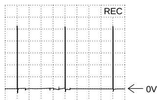
DC, 1V/Div, 5ms/Div IC7085-(6)
