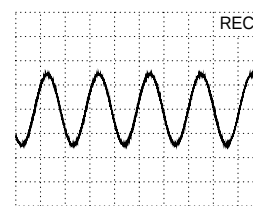
AC, 200mV/Div, 500μs/Div IC7400-(29)
