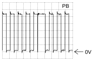
DC, 1V/Div, 2ms/Div IC7085-(12)
