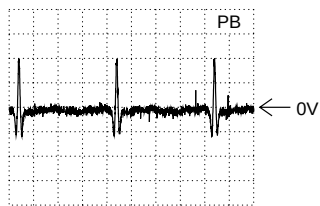
DC, 100mV/Div, 10ms/Div Connector 1501-(5)
