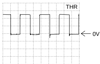
DC, 2V/Div, 20μs/Div IC7085-(10)
