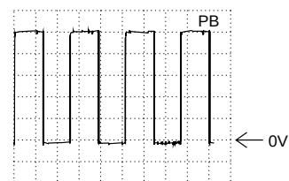
DC, 1V/Div, 10μs/Div IC7085-(25)
