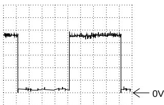
DC, 1V/Div, 5ms/Div IC7085-(36), LP Picture Search/Still
