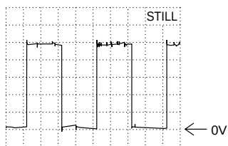
DC, 1V/Div, 10ms/Div IC7649-(5)
