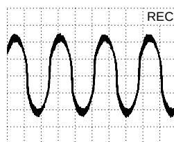
AC, 500mV/Div, 500μs/Div Connector 1502-(4)
