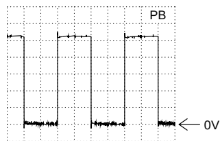
DC, 1V/Div, 10ms/Div IC7085-(20)
