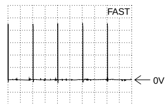
DC, 1V/Div, 10ms/Div Connector 1530-(9)
