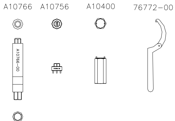
Figure 16: 79203-00 Tool Kit
