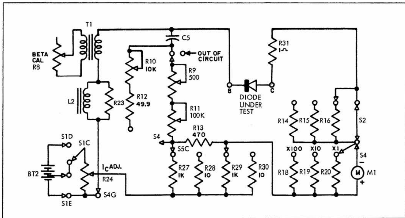
Figure 7. Diode Test Circuit
