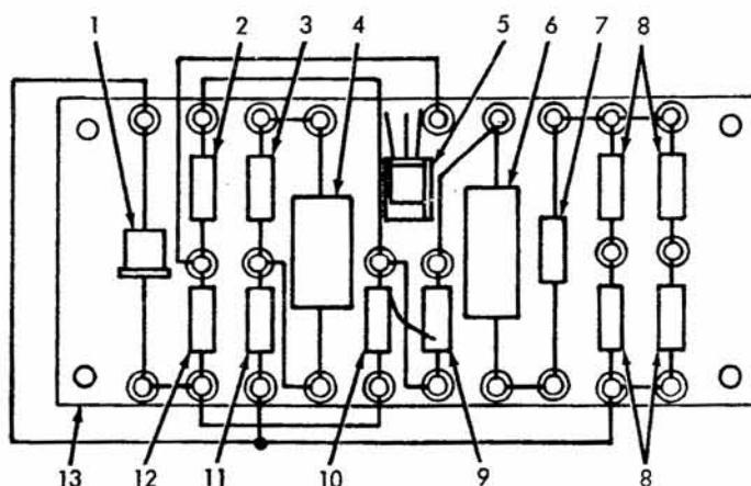
Figure 28. Terminal Board Assembly TB2
