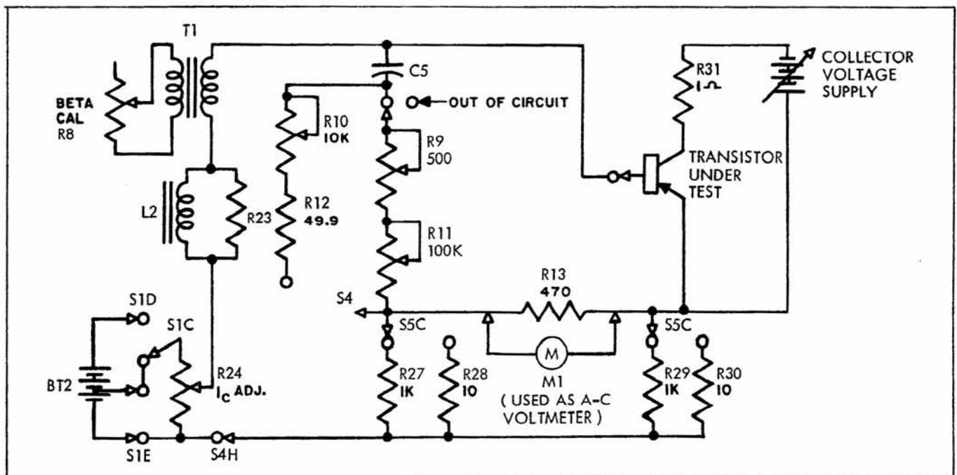
Figure 5. Z Ohms Test Circuit
