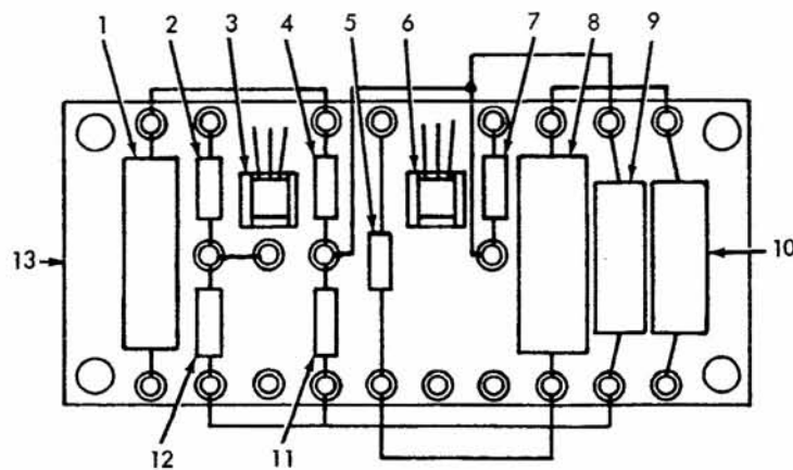
Figure 29. Terminal Board Assembly TB1
