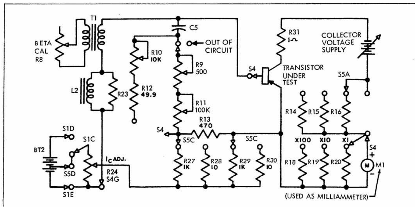
Figure 4. I_C Test Circuit
