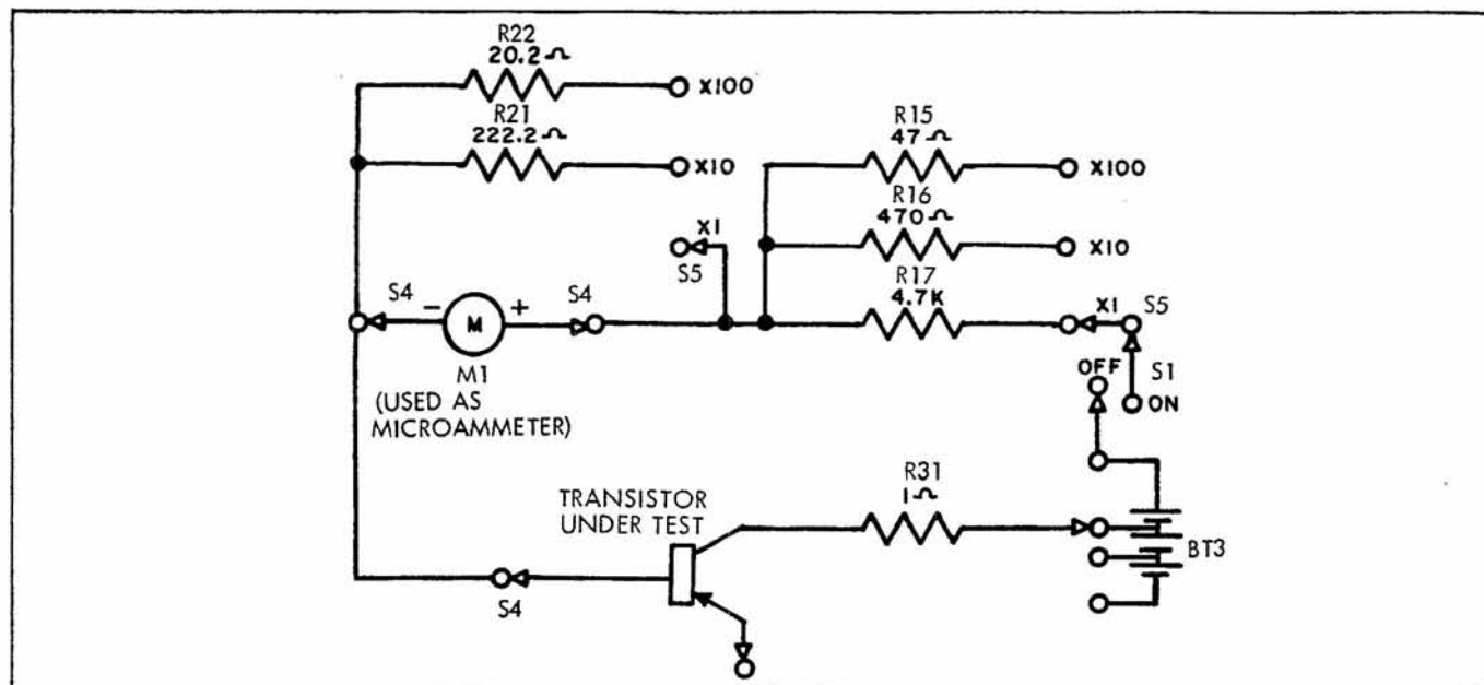
Figure 3. ICBO Test Circuit
