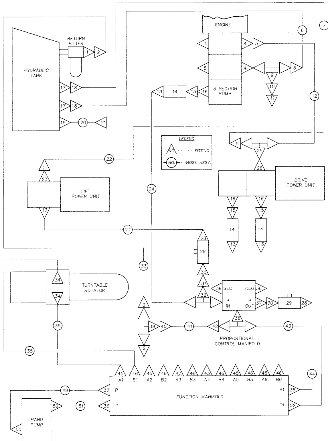
FIGURE 4-M
