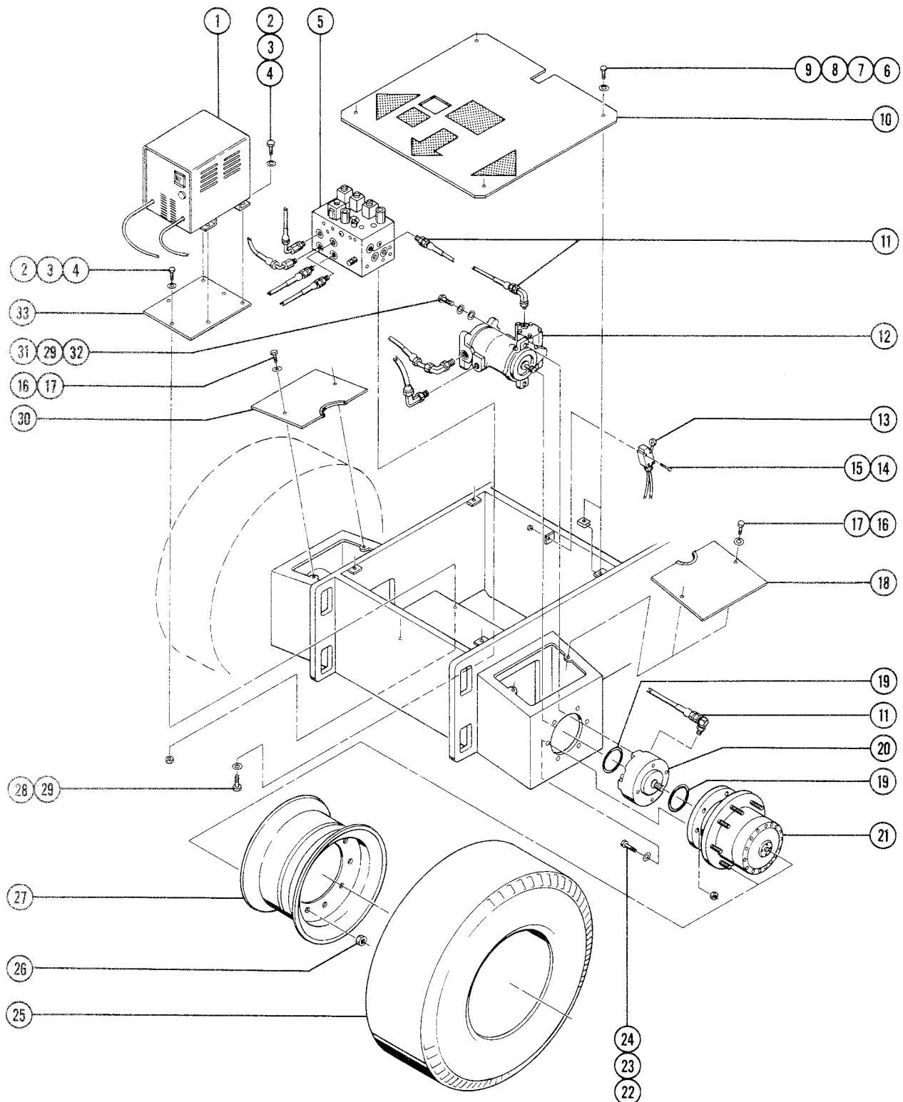
FIGURE 2-F
