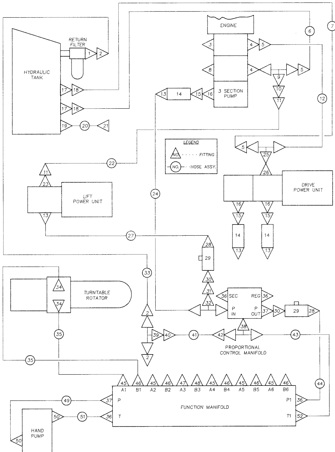
FIGURE 4-M
