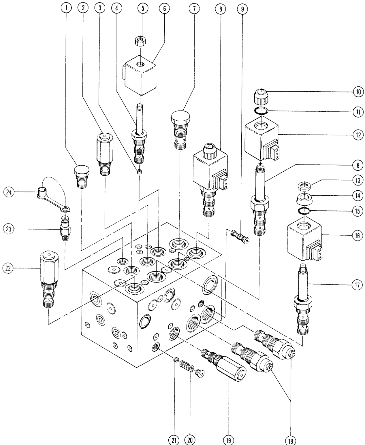
Figure 2-E Drive Manifold
