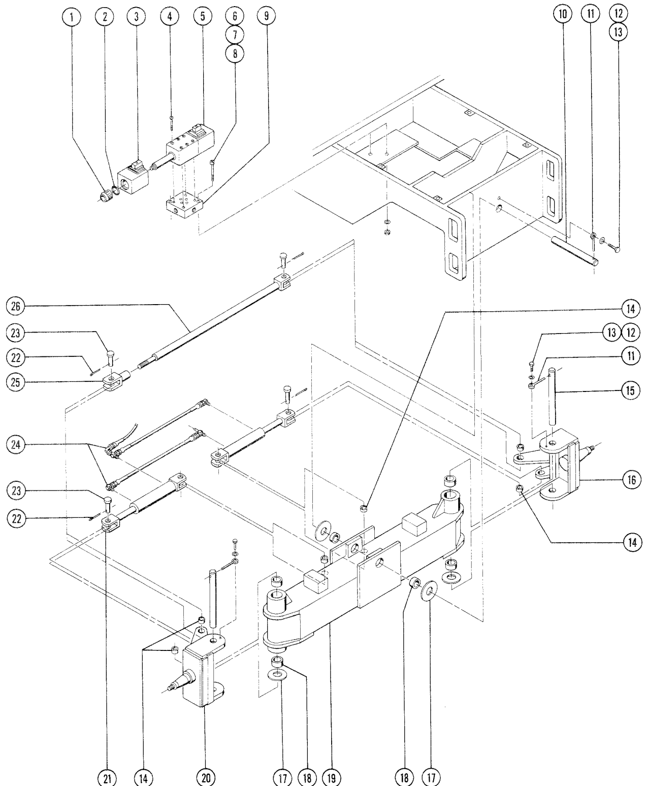
Figure 2-A Steer Linkage
