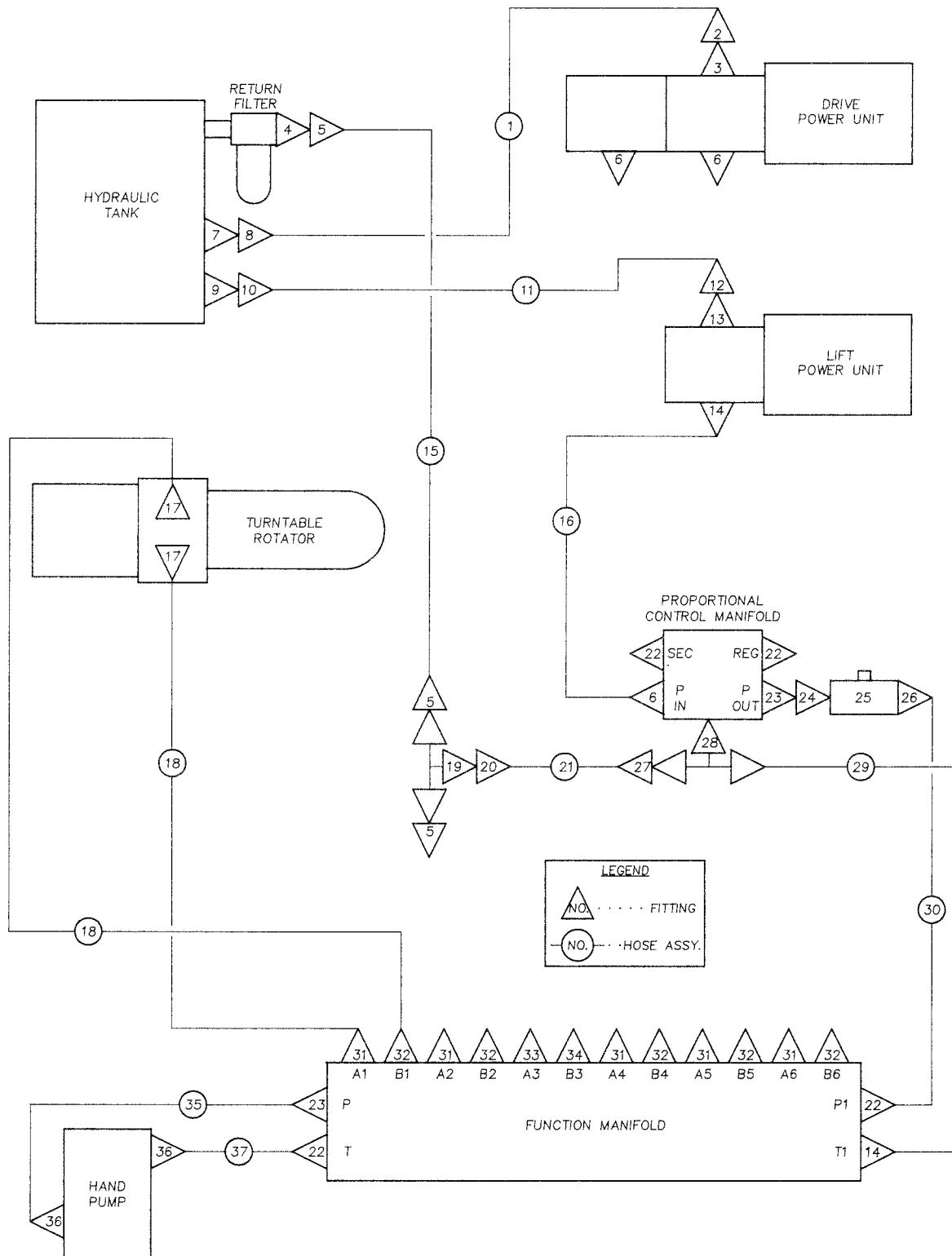
Figure 4-L Hydraulic Hoses and Fittings DC Models
