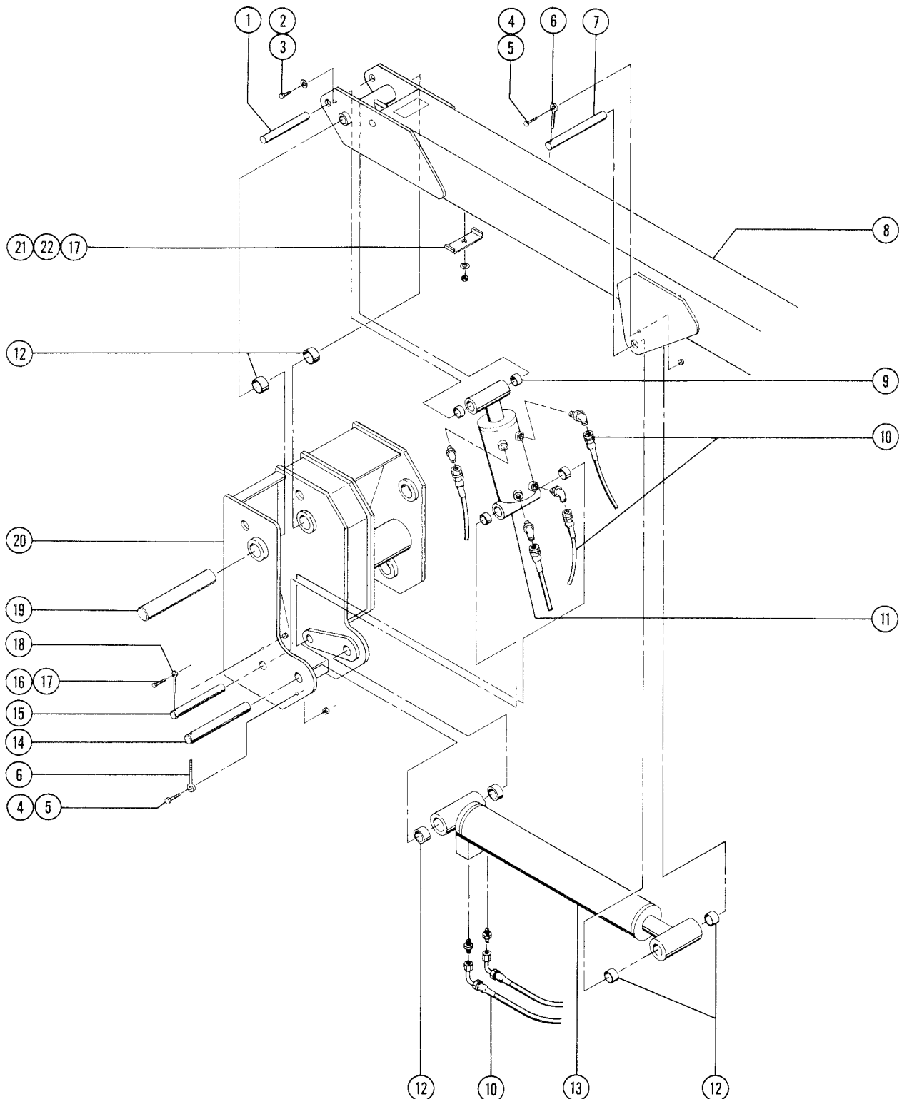
Figure 5-C Upper Mid-pivot
