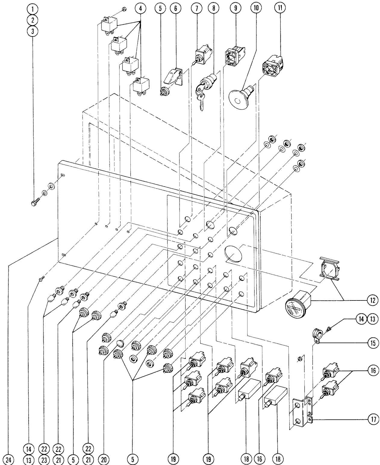
Figure 4-I Ground Controls - View 2
