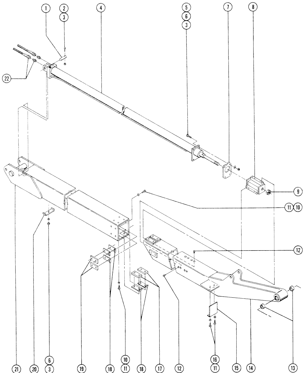
Figure 5-D Primary and Extension Booms
