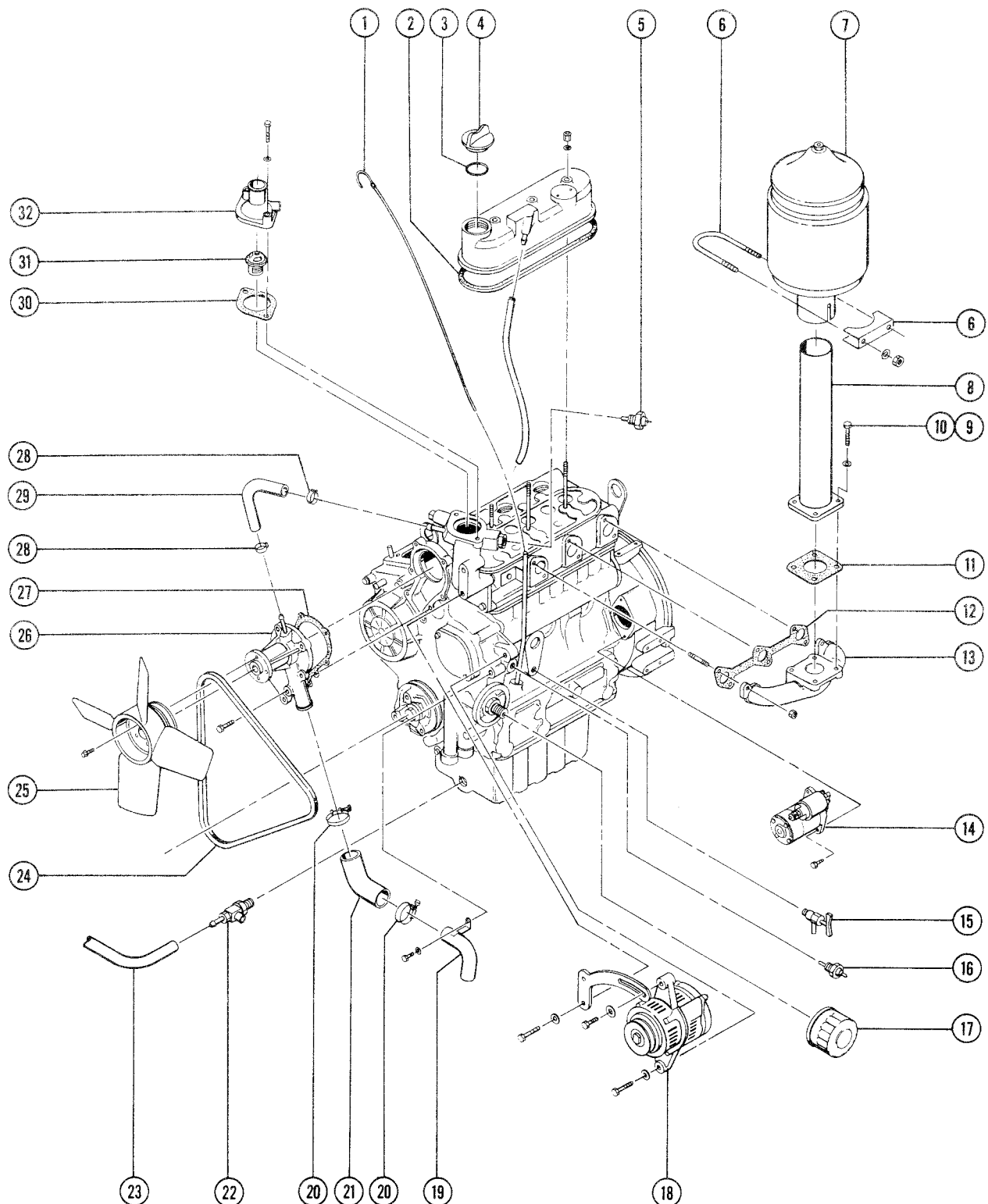
FIGURE 3-H
