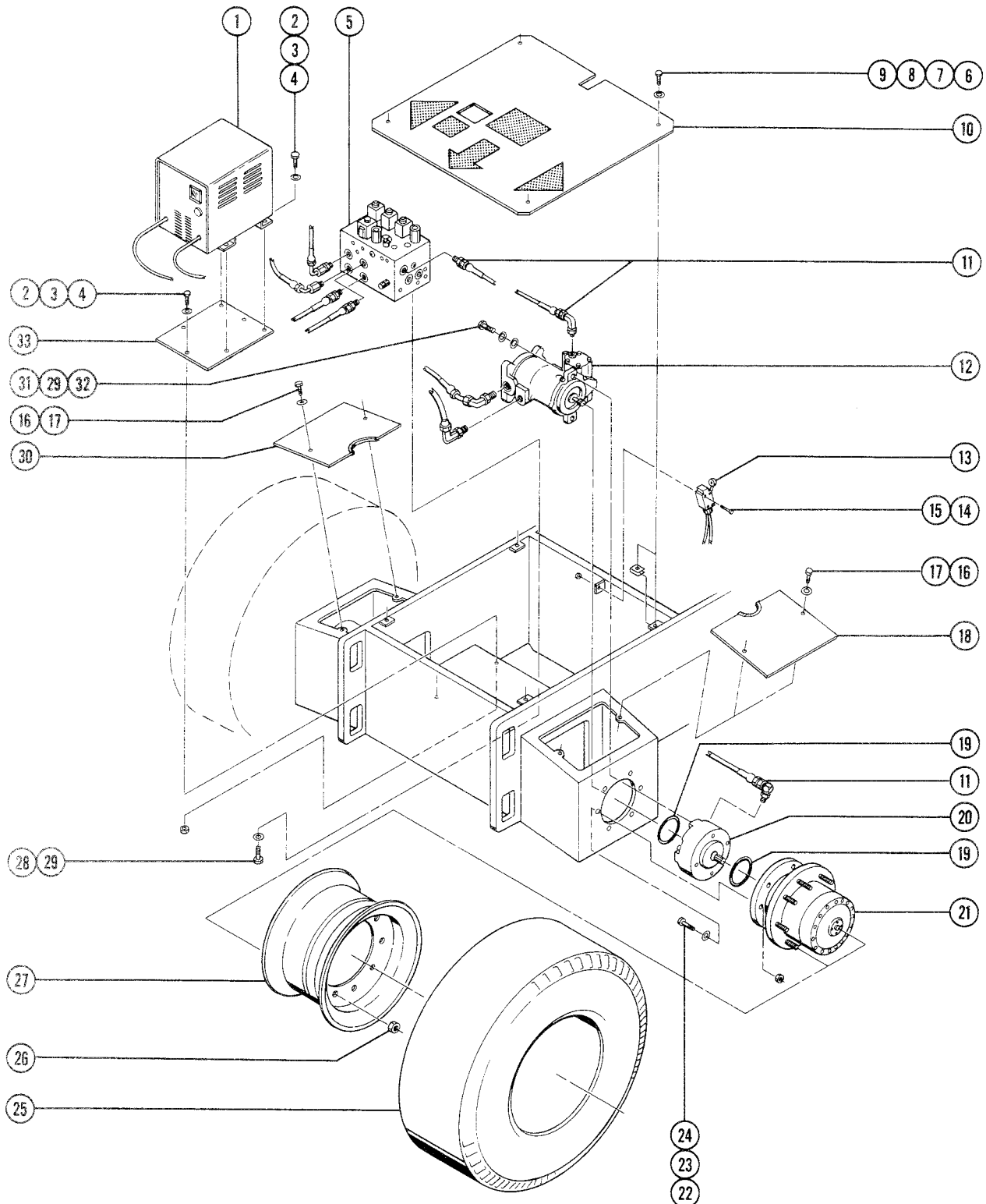
Figure 2-F Non-steer Axle
