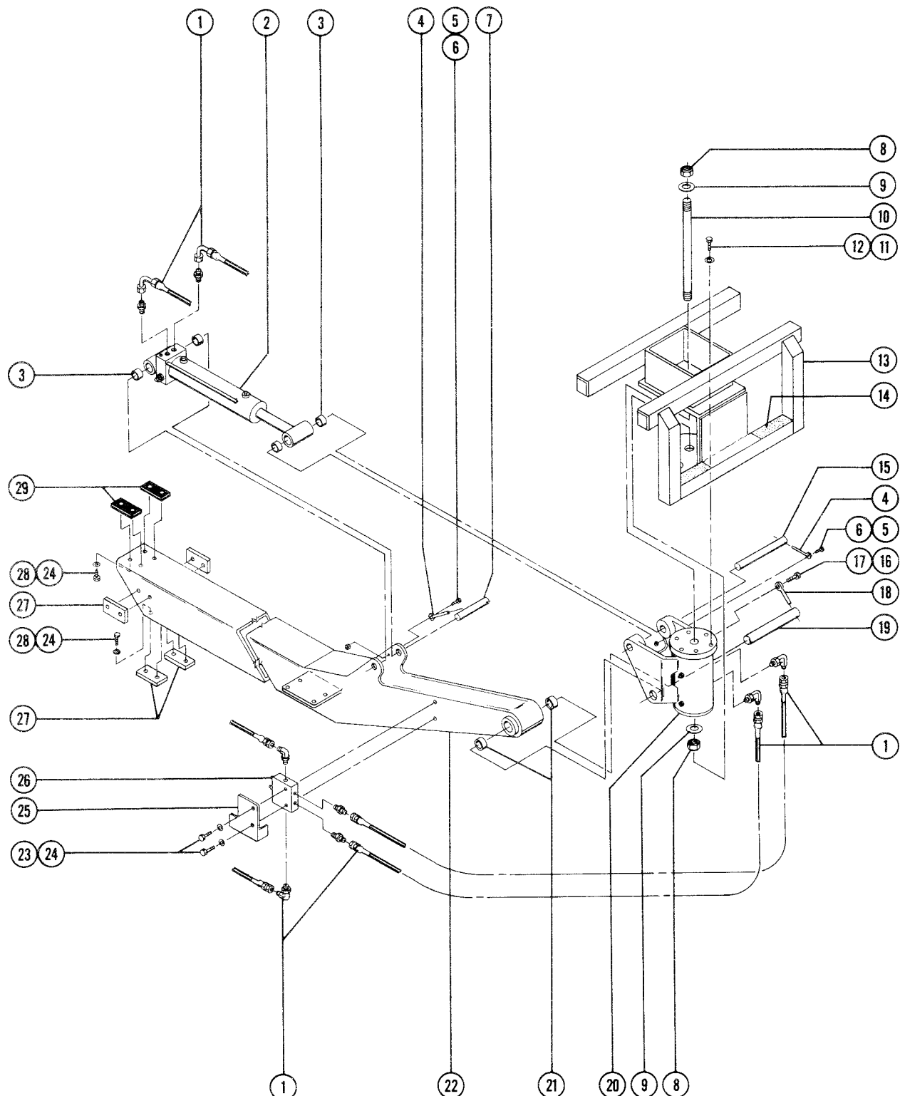
Figure 5-F Platform Leveling and Rotation
