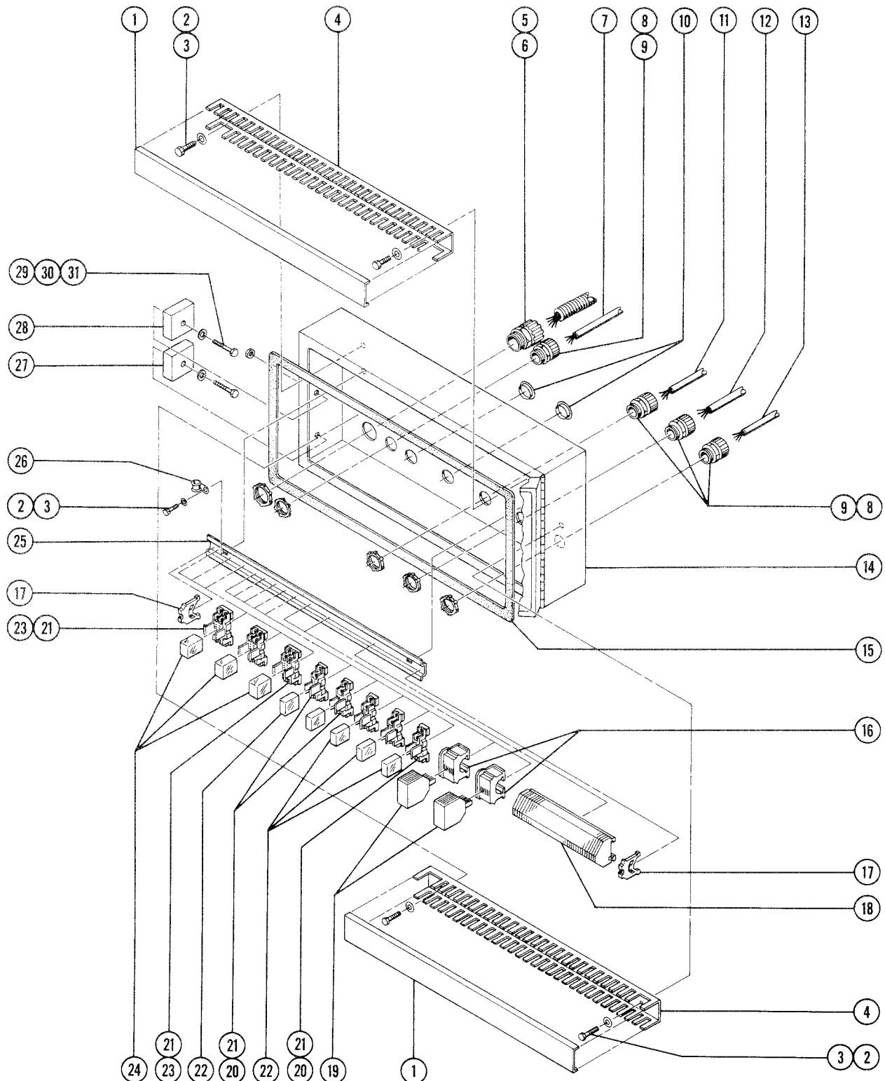
Figure 4-H Ground Controls - View 1
