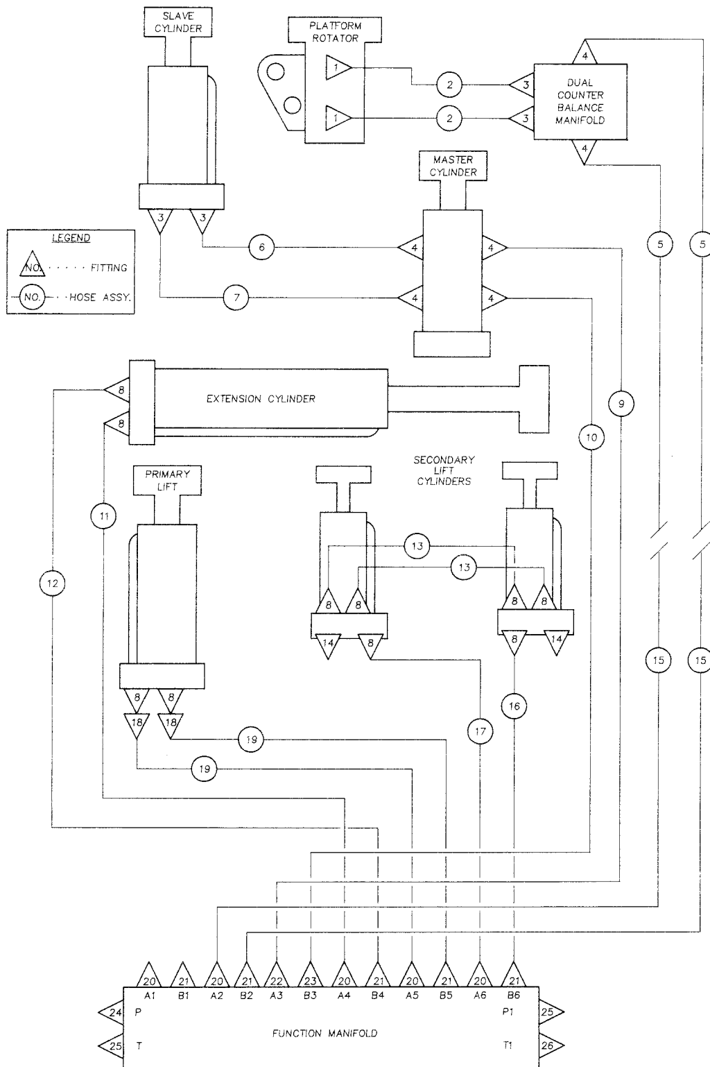
Figure 5-G Hydraulic Hoses And Fittings
