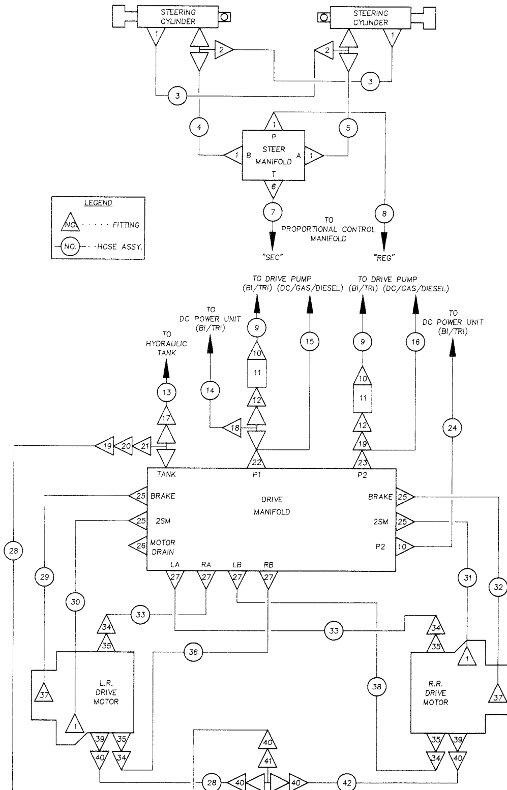
Figure 2-G Hydraulic Hoses and Fittings
