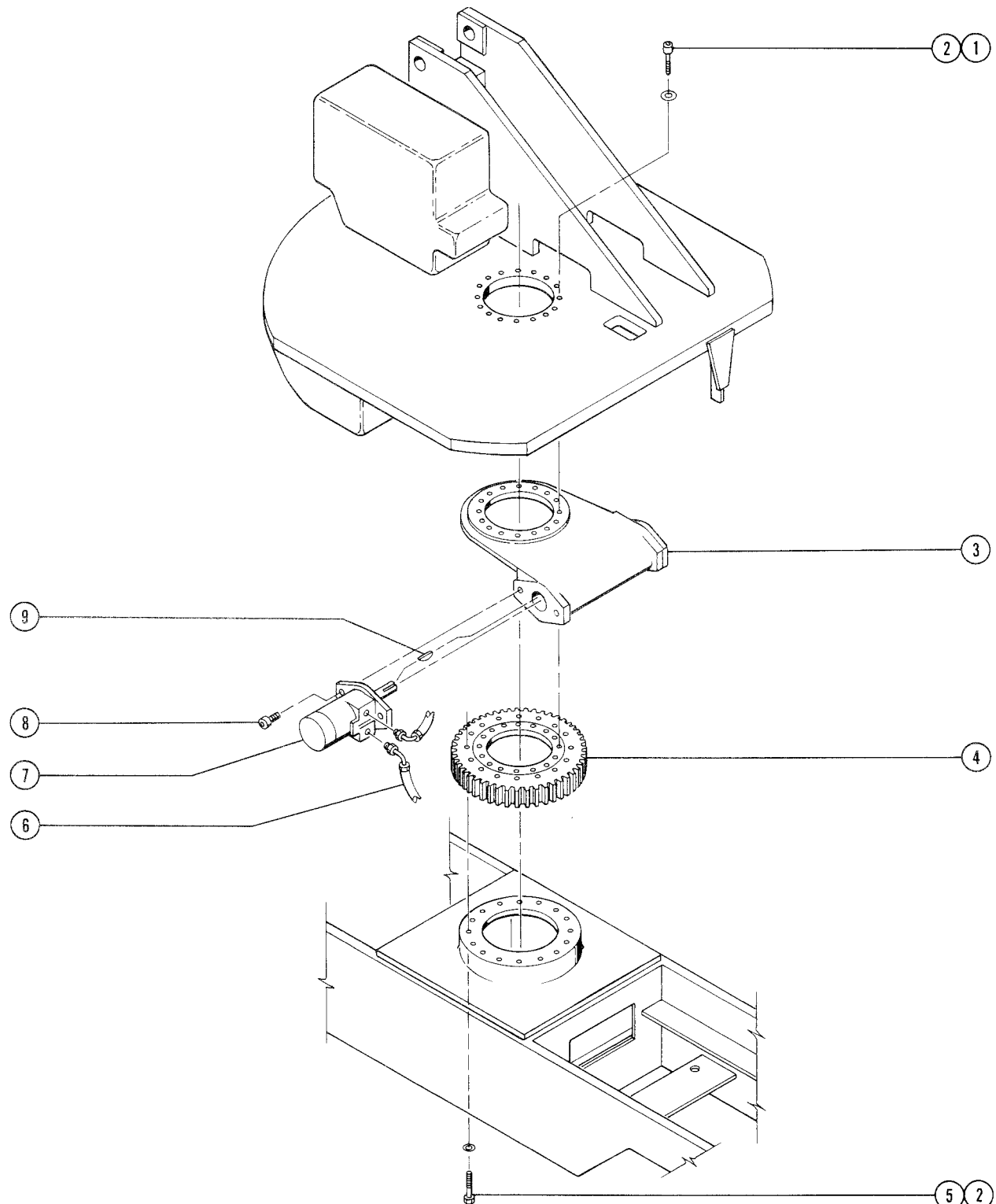
Figure 4-A Turntable Rotator
