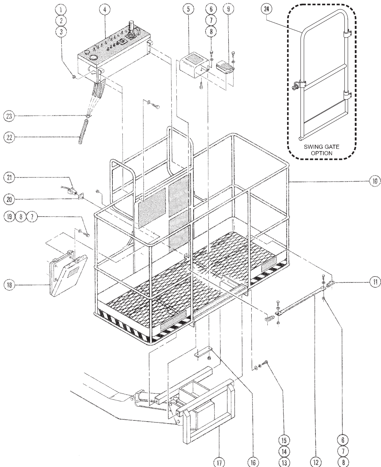
Figure 6-A Platform
