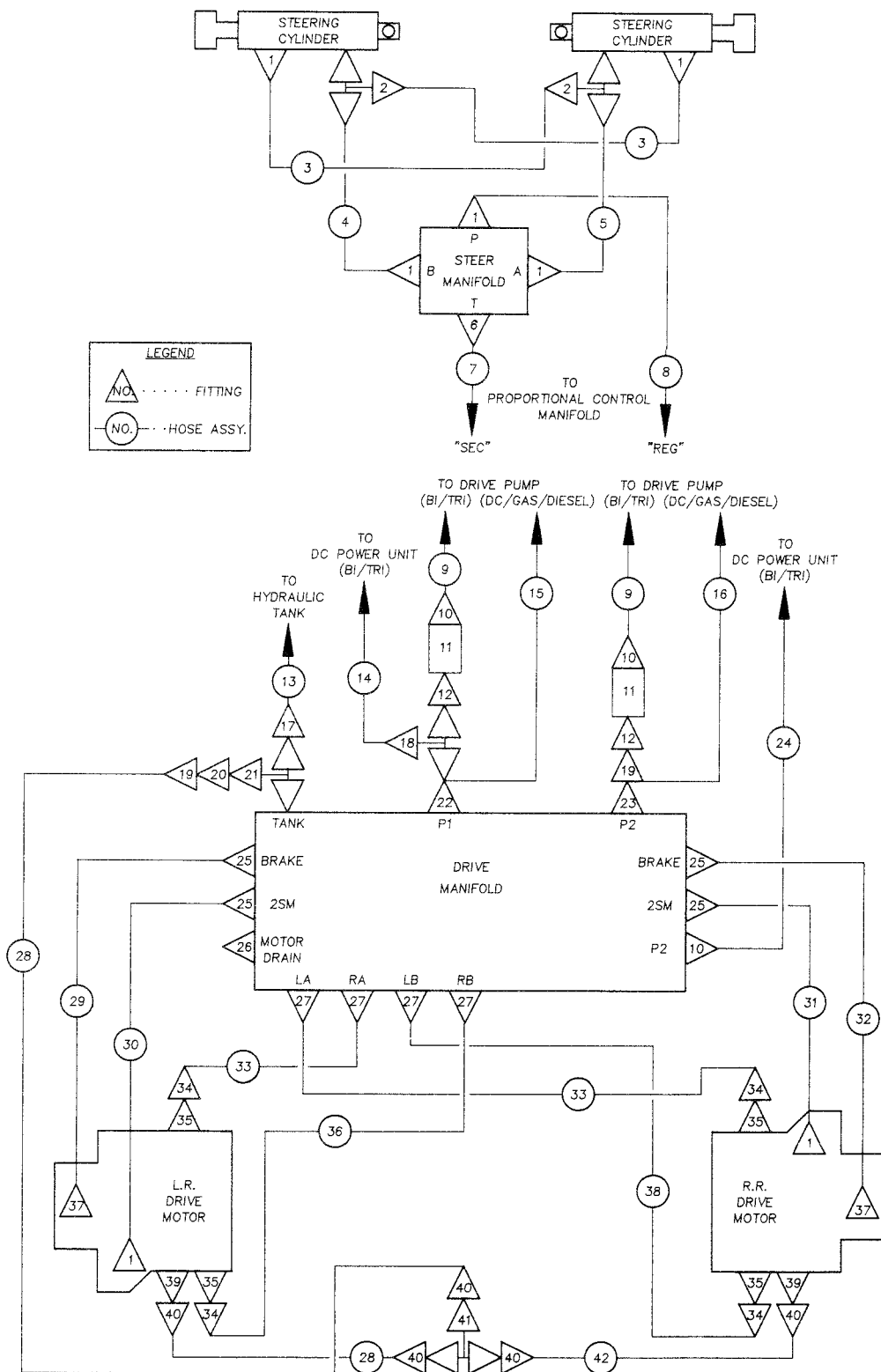
FIGURE 2-G
