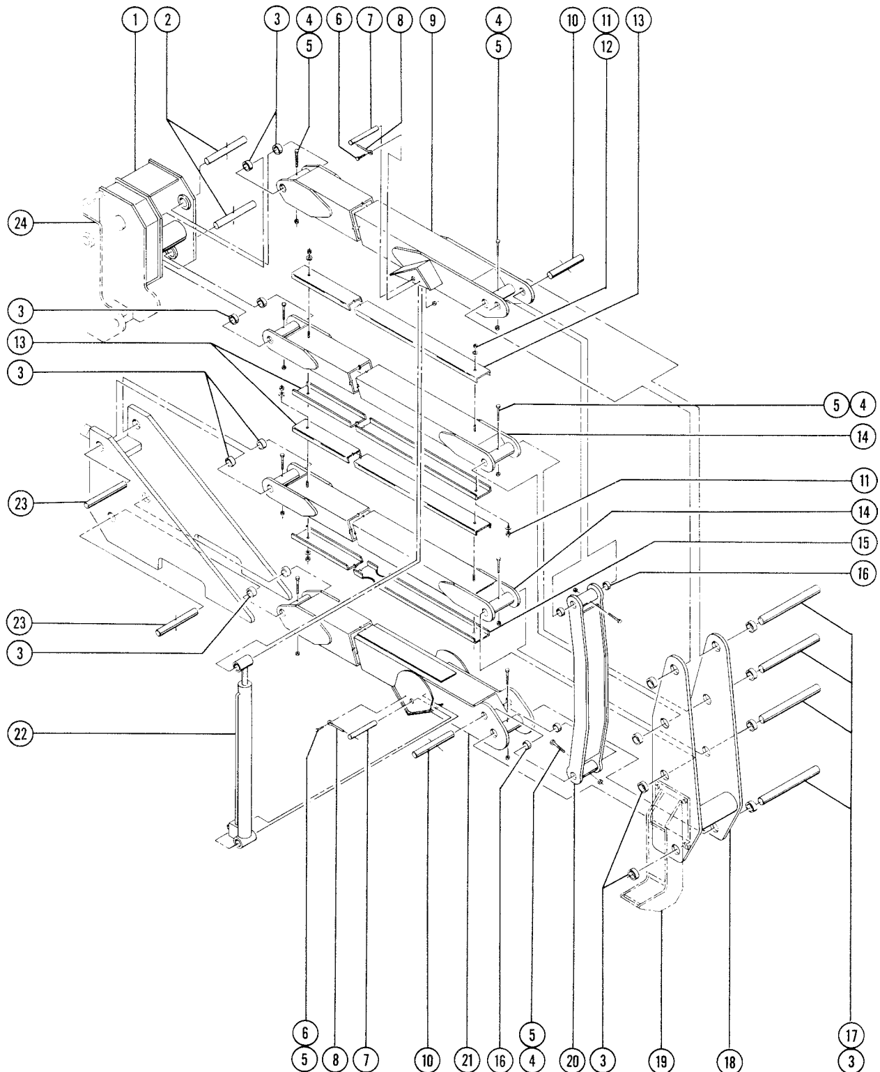
Figure 5-A Secondary Boom
