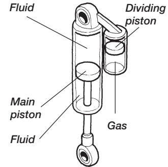
2. External gas reservoir piggyback
