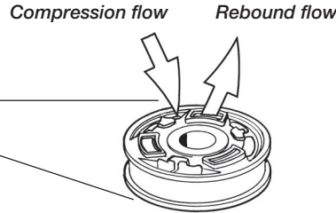
Fig 2. Piston with aperture
