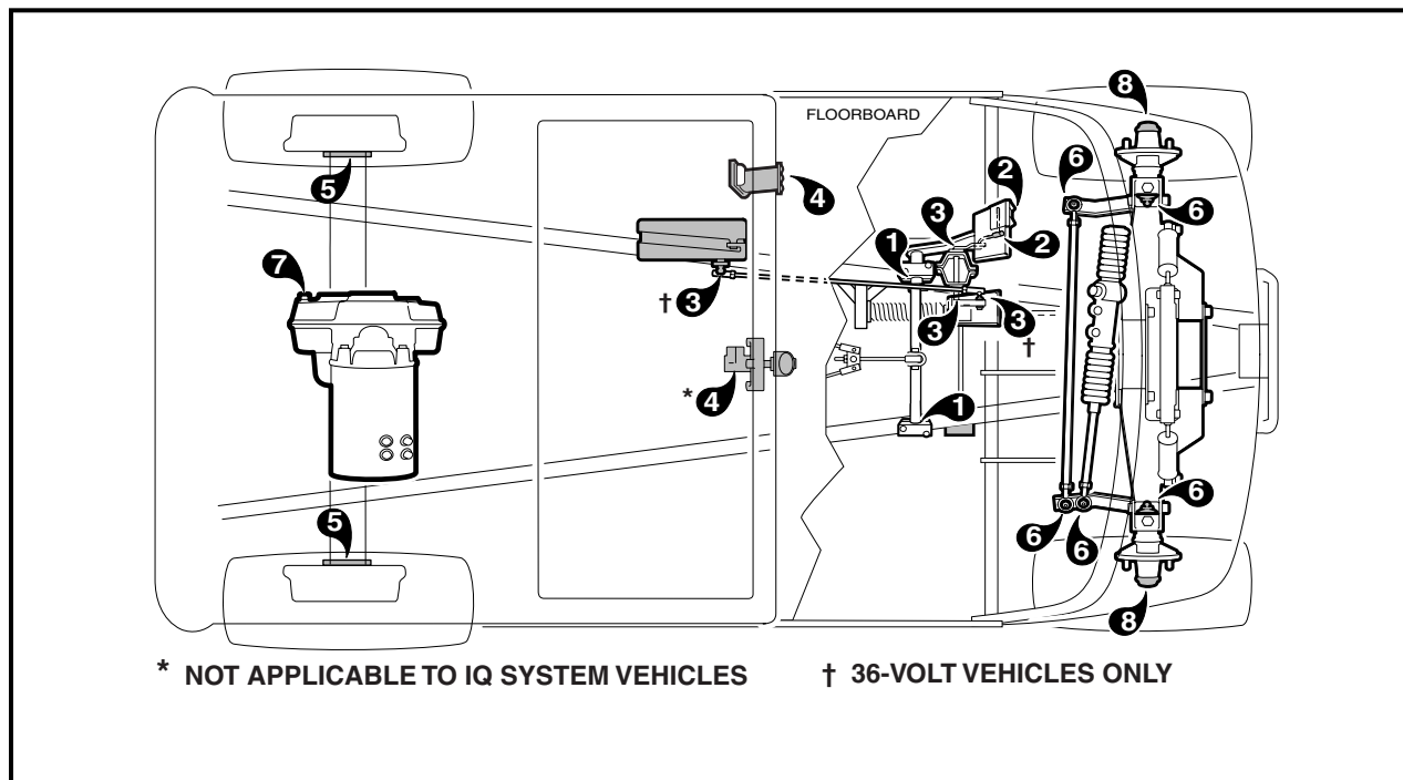
Figure 12 Lubrication Points
