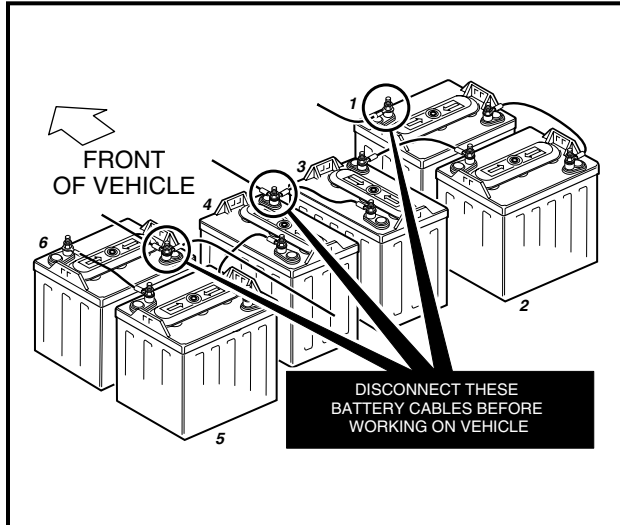
Figure 1 V-Glide 36-Volt Vehicle
