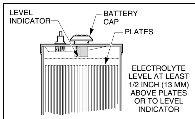
Figure 13 Battery Electrolyte Level
