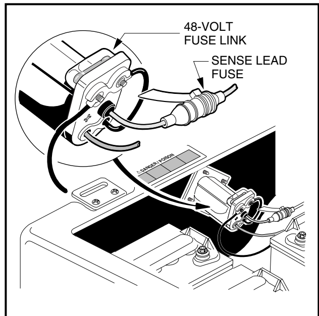
Figure 17 Receptacle Fuse Link for 48-Volt and IQ System Vehicles
