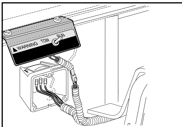
Figure 11 Tow/Run Switch
