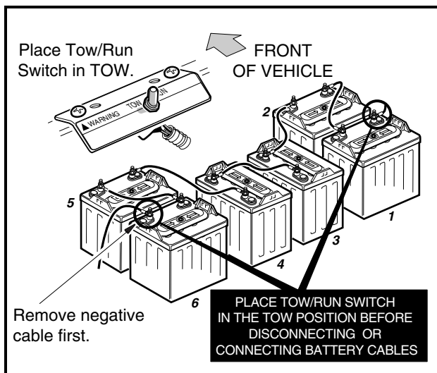
Figure 3 IQ System Vehicle
