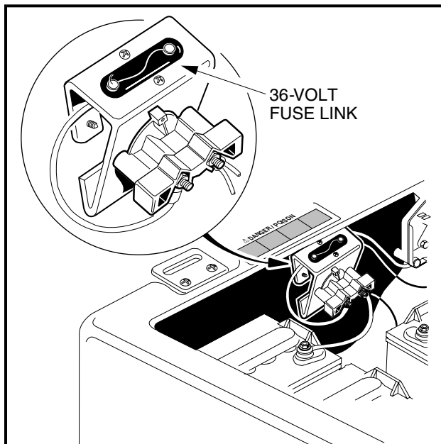
Figure 16 Receptacle Fuse Link for 36-Volt Vehicle
