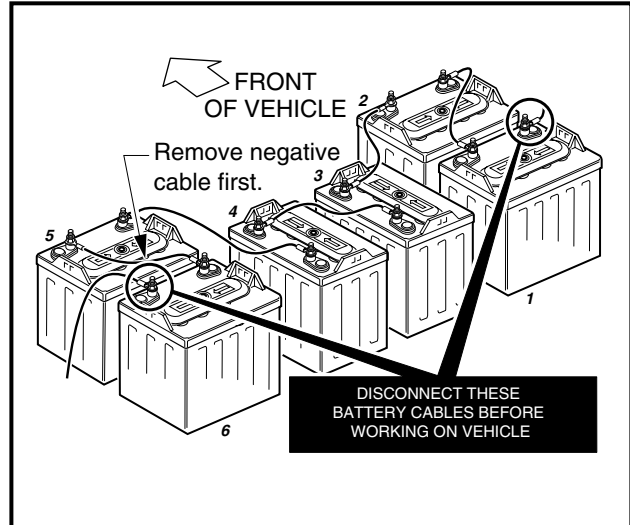
Figure 2 PowerDrive System 48 Vehicle
