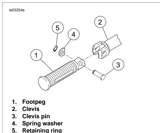
Figure 1. Footpeg Removal/Install (generic footpeg shown)
