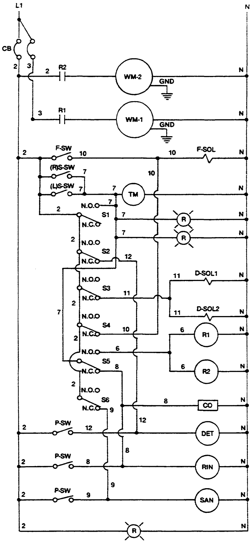
CONSERVER II SINGLE PHASE 115 VOLTS
