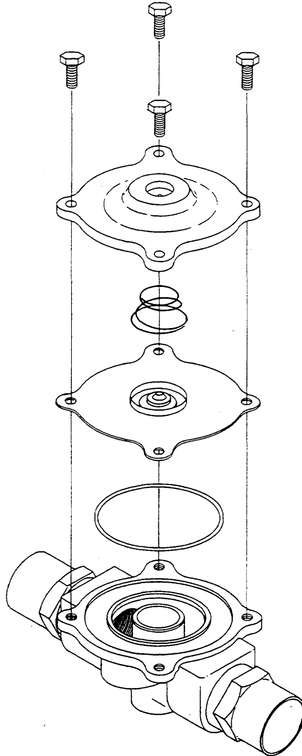
ANTI-FOAM VALVE 3/4" ASSEMBLY P/N 0185500 DIAPHRAGM KIT 0185501
