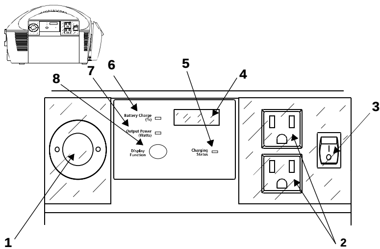
XPower Powerpack Features
