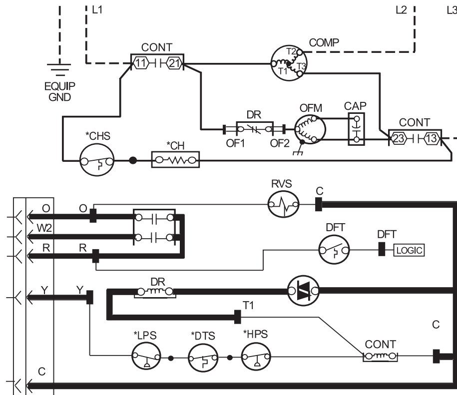
Fig. 14 – 25HHA4/224ANS Wiring Diagram 208/230V 3 Phase
