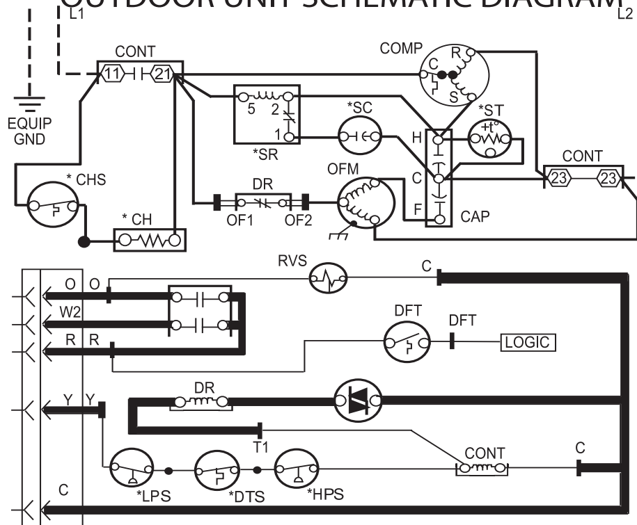
Fig. 13 – 25HHA4/224ANS Wiring Diagram 208/230V 1 Phase
