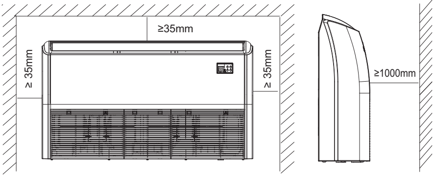
Fig. 5 – 40MKCB**F, 40MKQB**F Unit Clearance
