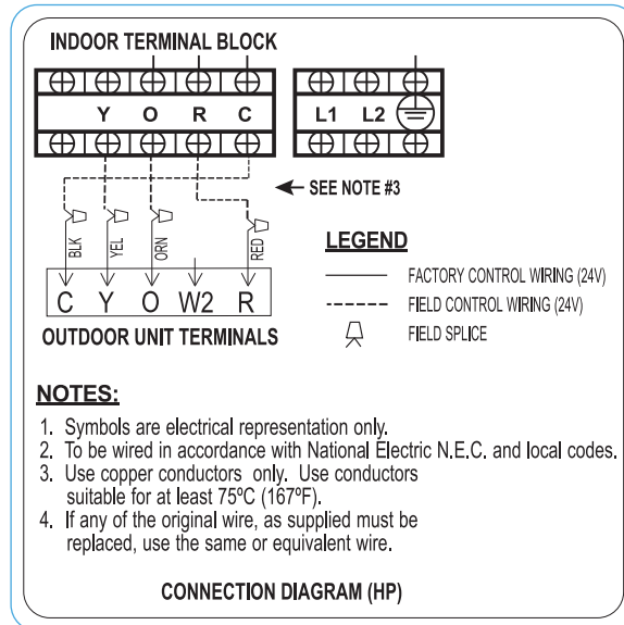
Fig. 8 – 40MKQB**F / 25HHA4 or 224ANS Connecting Diagram
