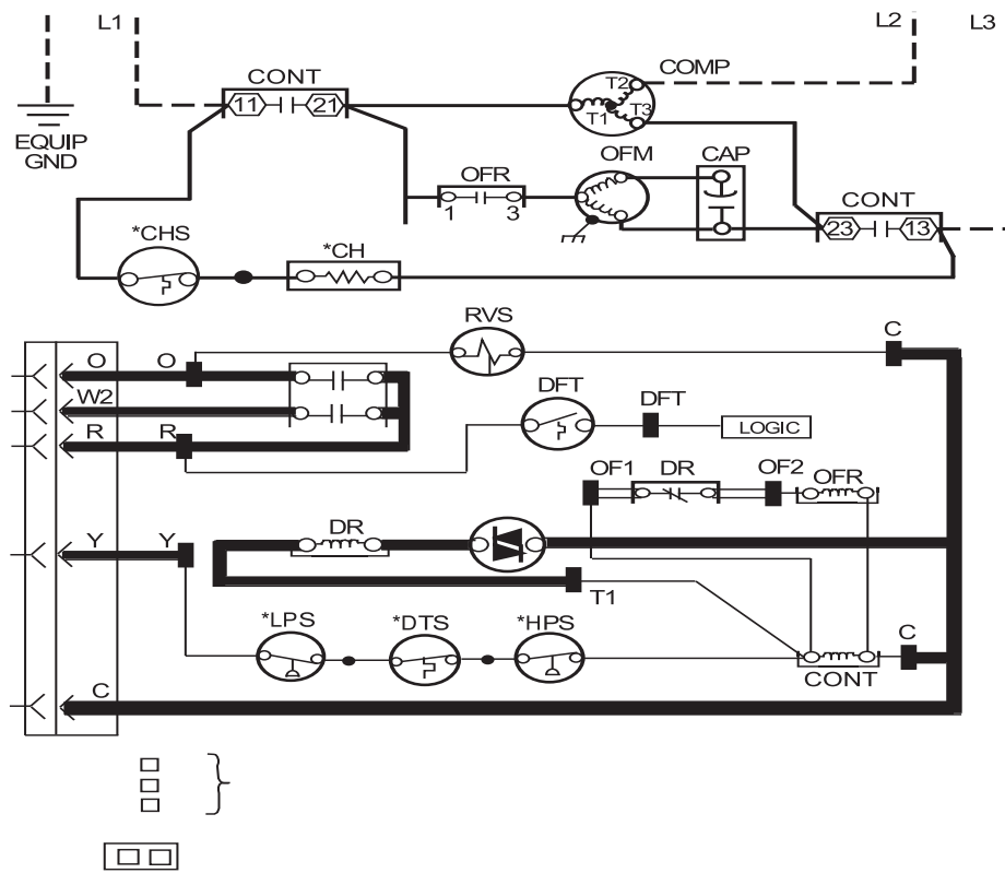
Fig. 15 – 25HHA4/224ANS Wiring Diagram 460V 3 Phase
