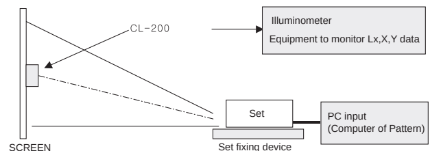
<Fig.8-1> Device setting diagram for CWI adjustment
