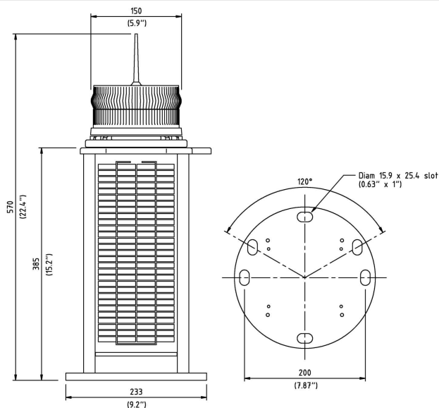
Fig 1. SLC420 Solar Marine Lantern
