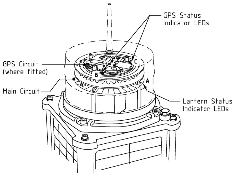
Fig 3. SLC420 Lantern Status
