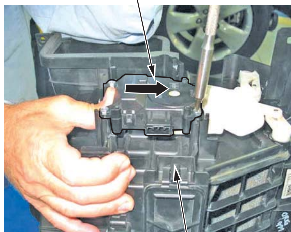
NEW BLOWER UNIT
