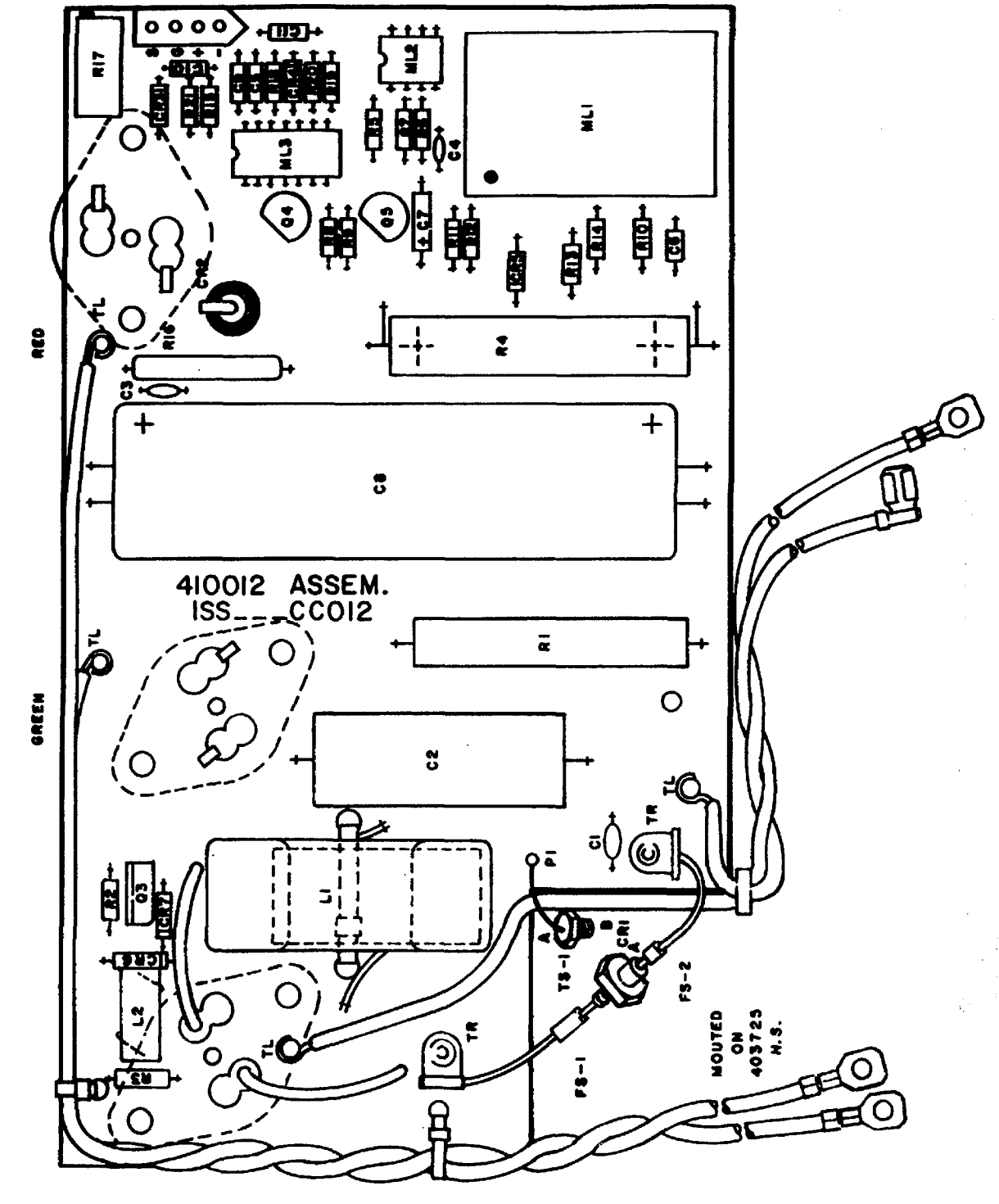
Component Layout of 410012 Circuit Card
