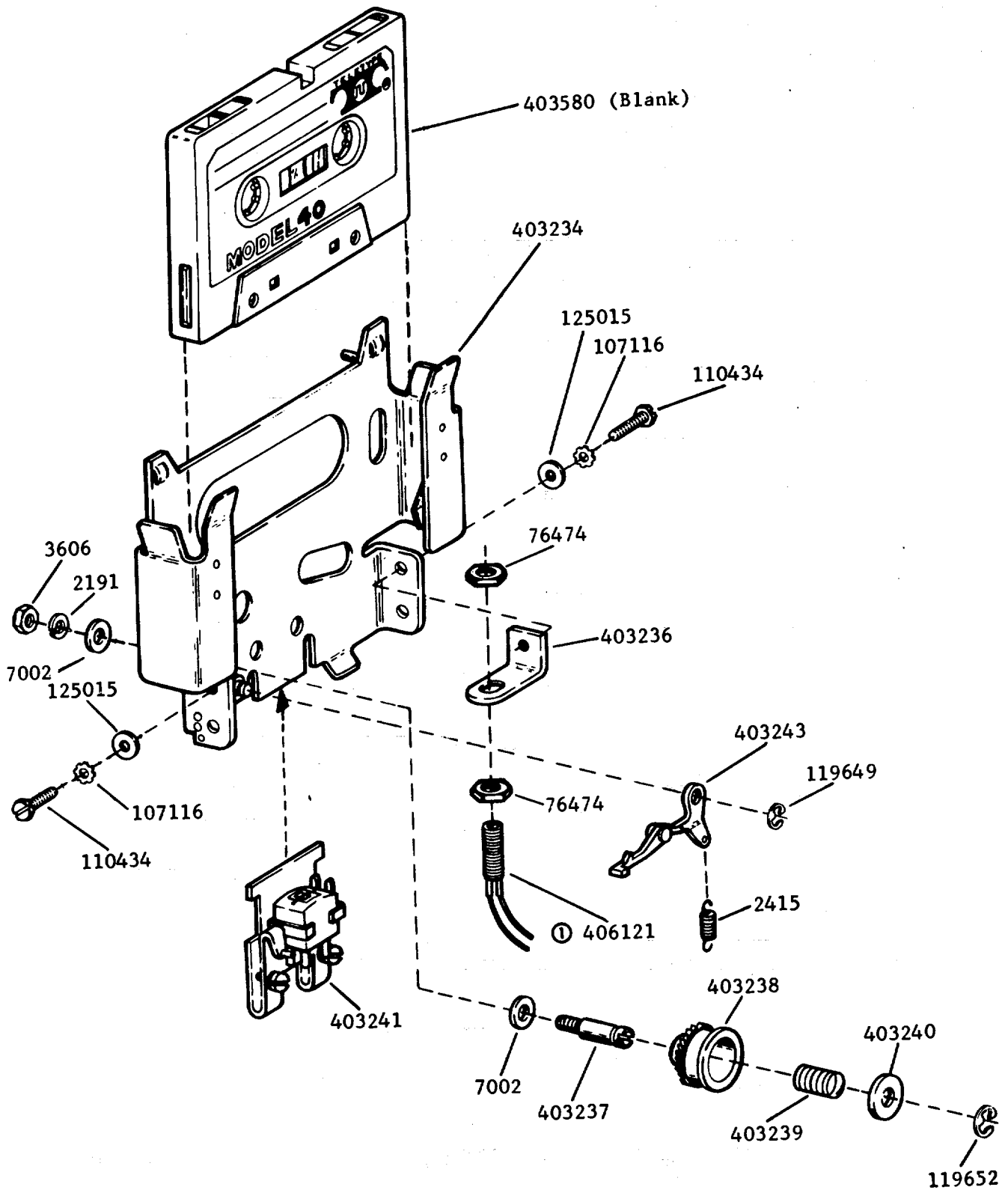
Cassette Holder Assembly
