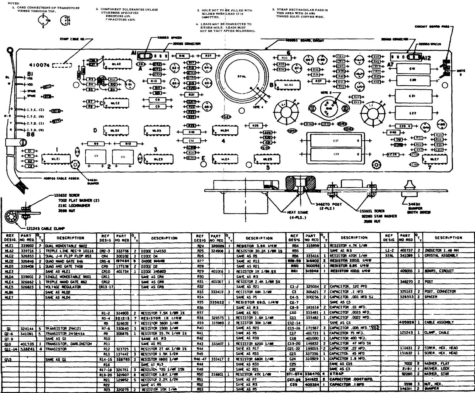
410074 Circuit Card (Early Design)
