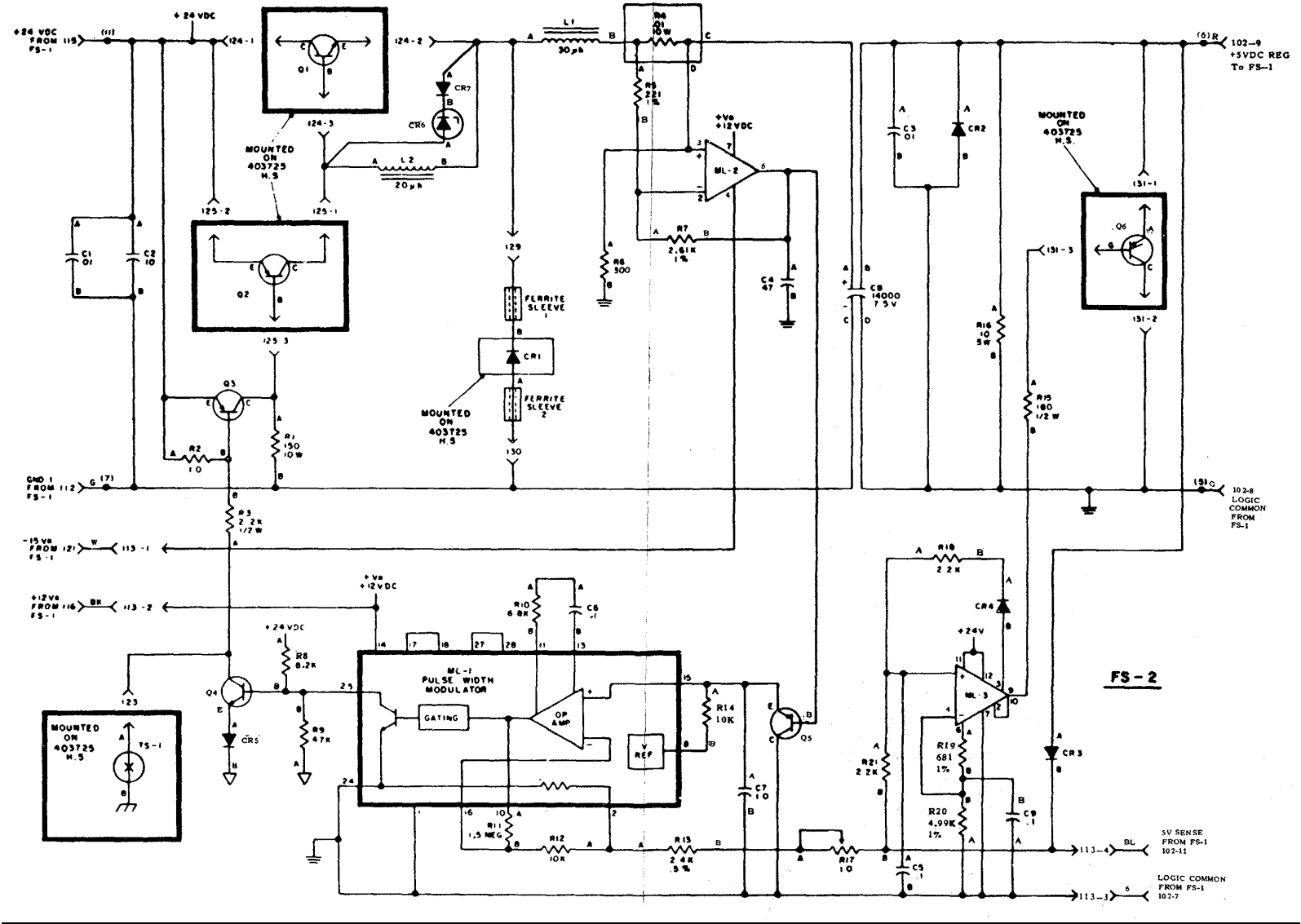
Functional Schematic of 410012 Circuit Card
