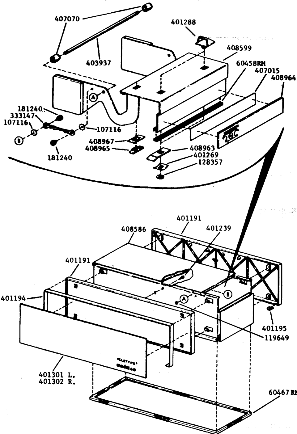
40CAB102- Upper Cabinet Assembly
