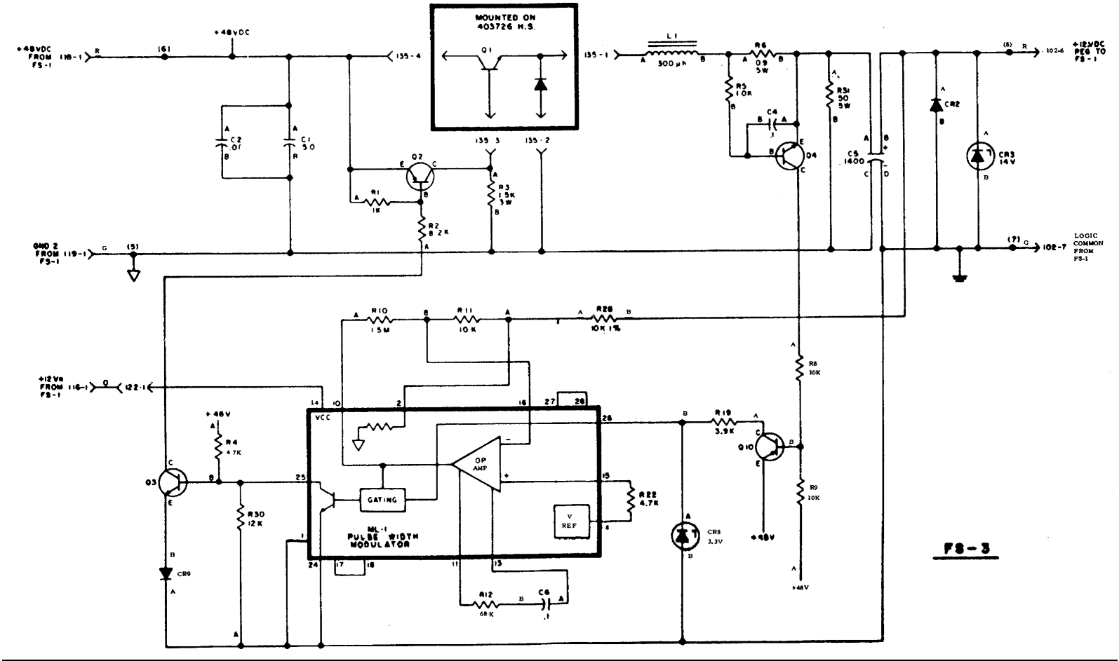
Functional Schematic of +12 V dc Circuit on 410011 Circuit Card
