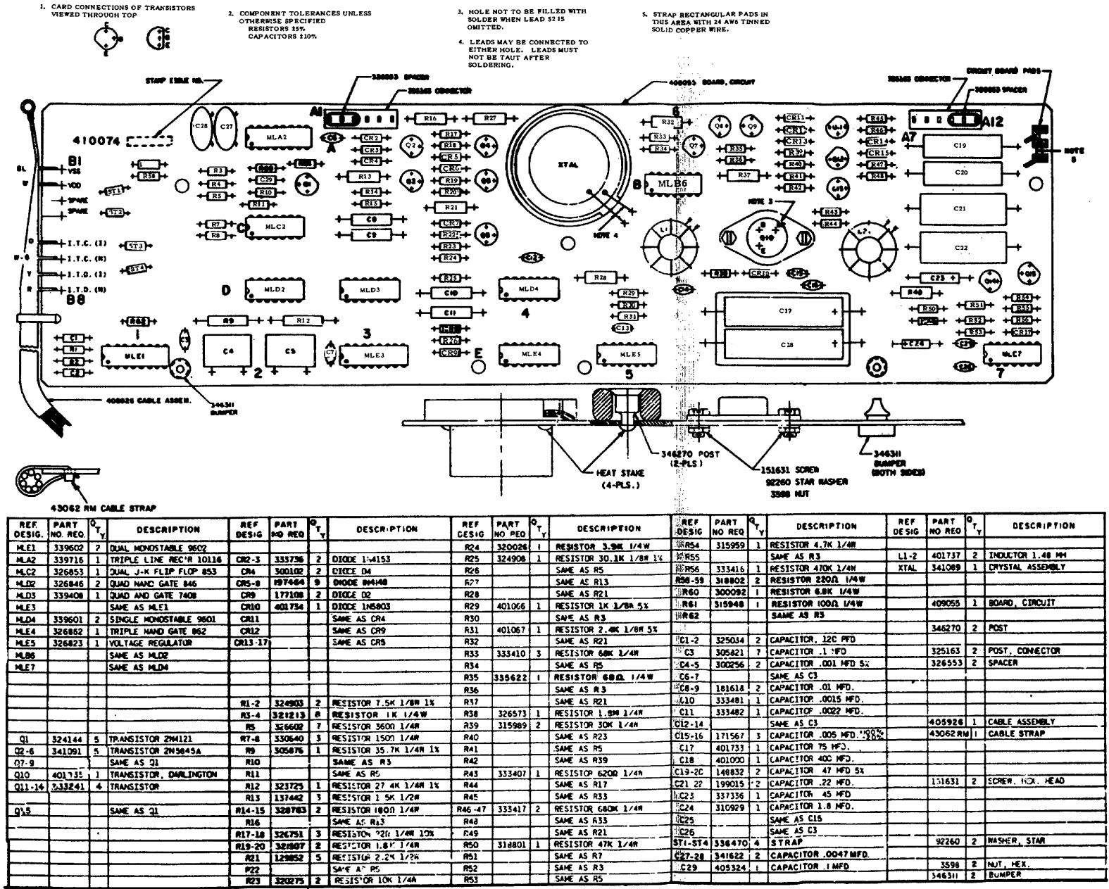
410074 Circuit Card (Late Design)
