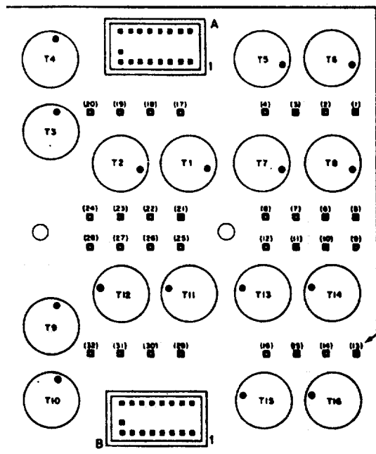
410157 CIRCUIT CARD
