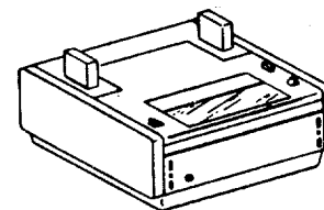
40CAB252/RA Monitor and Opcon Mounting
