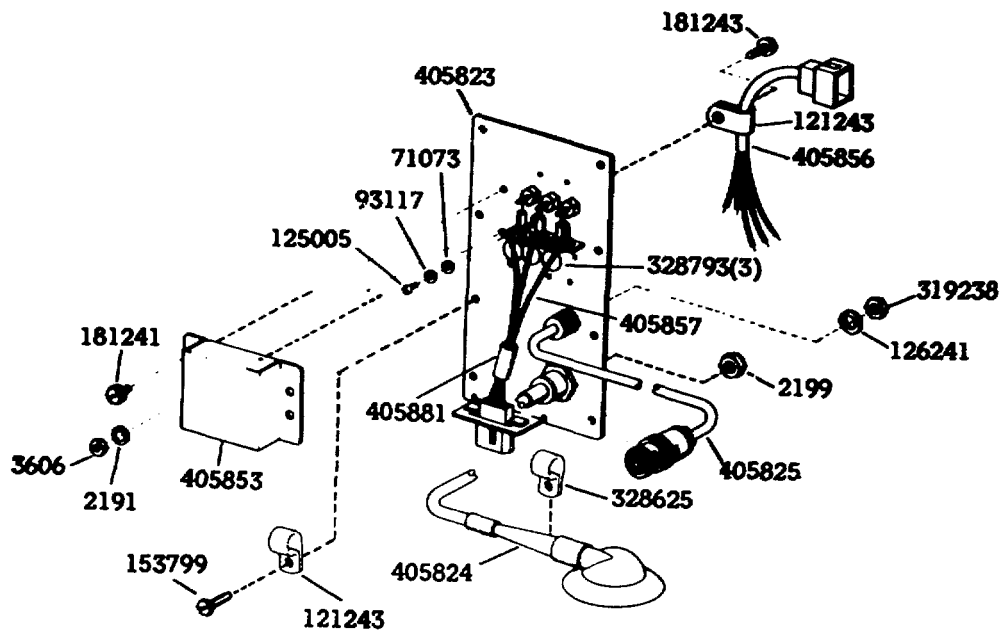
HIGH VOLTAGE PLATE ASSEMBLY (405859)
