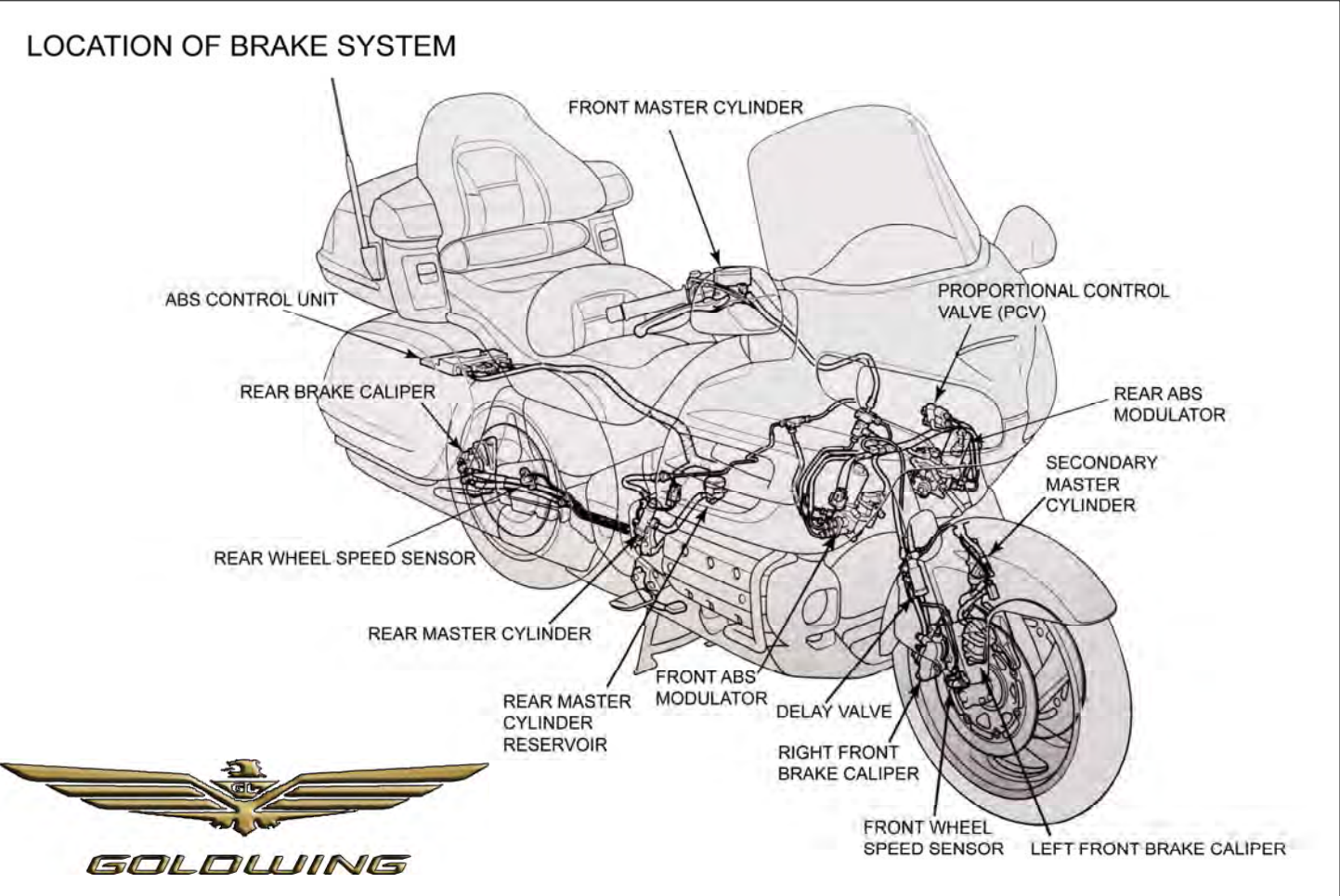
(Fig: Location of Brake System) This is provided as a Legend guide, technical name and location on bike.
