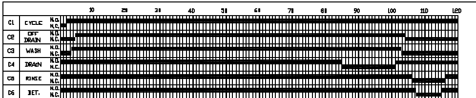
TIMING CHART
