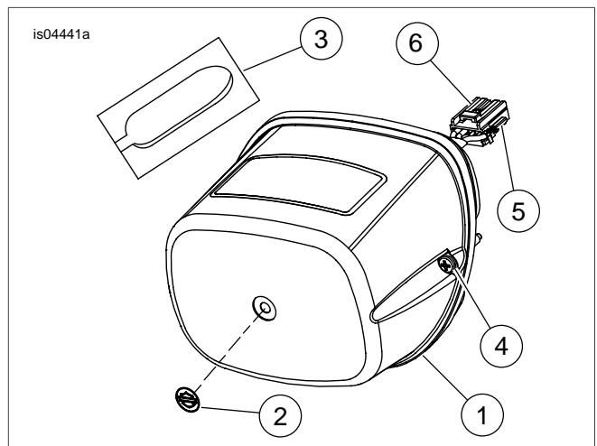
Figure 3. Service Parts: LED Tail Lamp with Bar & Shield Logo (Non-FLHX Model Shown)
