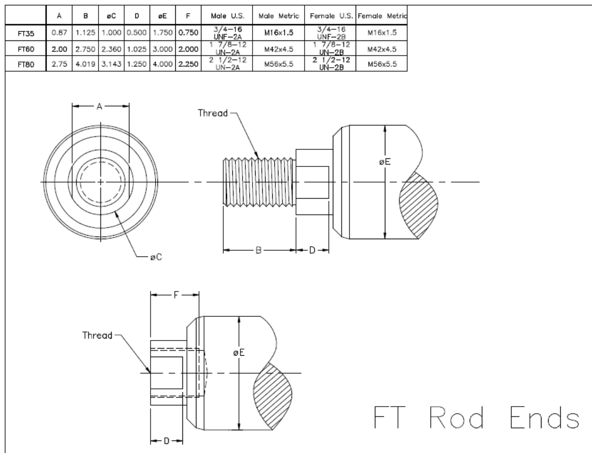
Figure 16: FT Rod End Thread Details
