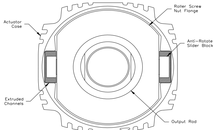
Figure 5: Anti-Rotate Mechanism
