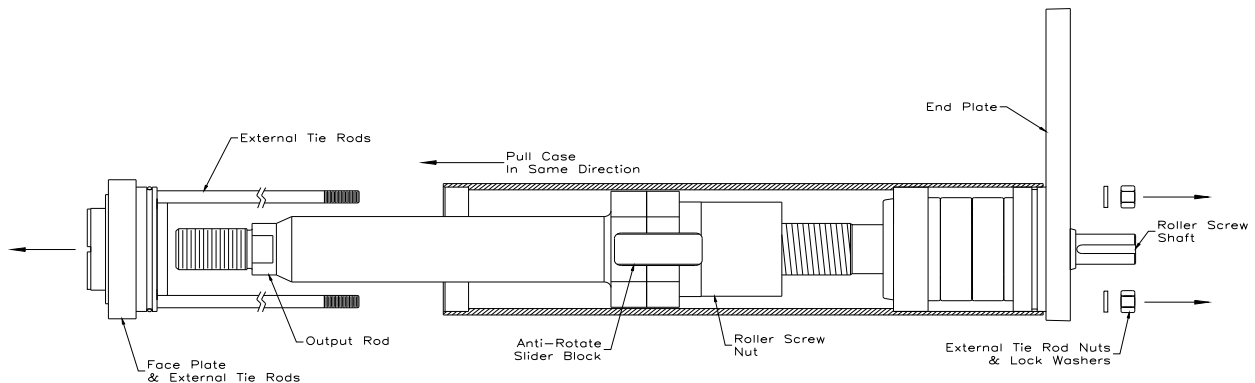
Figure 13: Actuator Disassembly
