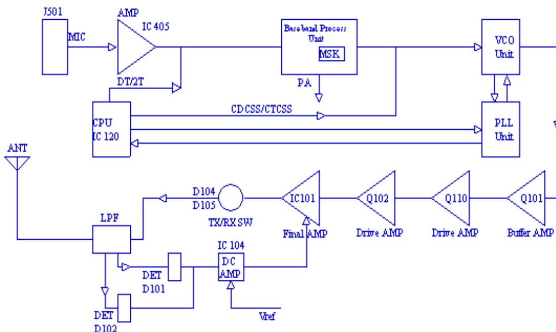
Fig. 2 Transmitter Circuit
