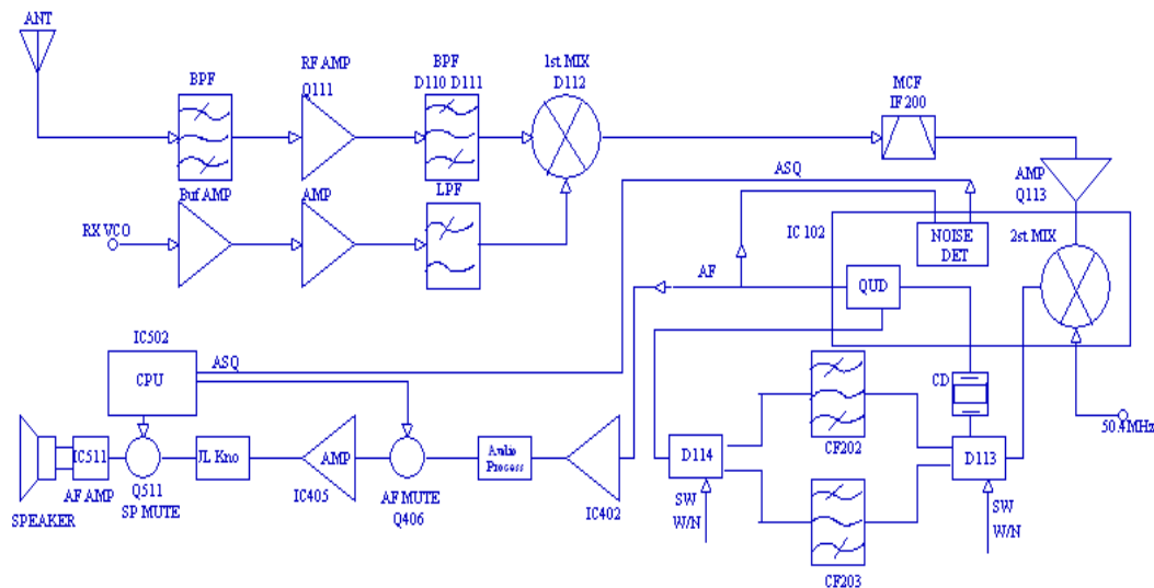
Fig. 1 Receiver Circuit
