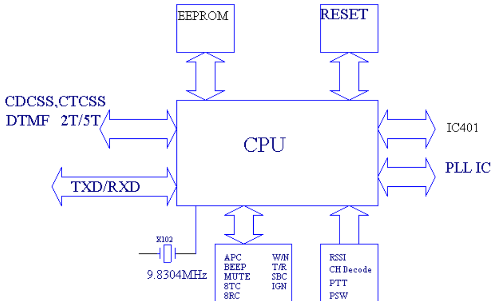
Fig. 4 Control Circuit
