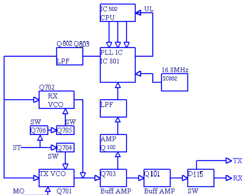
Fig. 3 PLL Circuit
