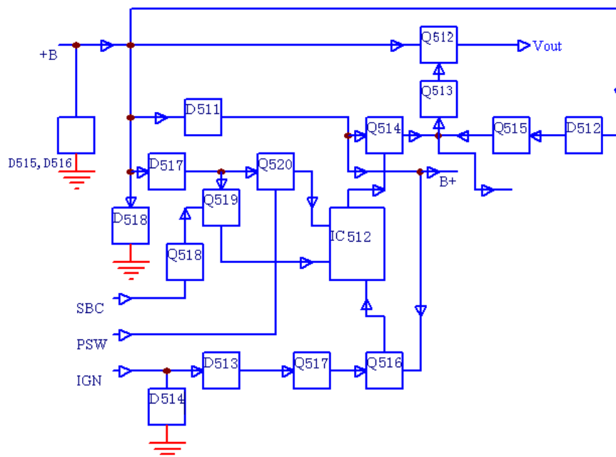
Fig. 5 Power Supply Circuit
