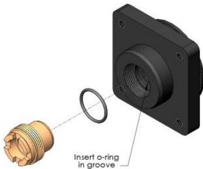
Main Rod Seal Gland and Bushing
