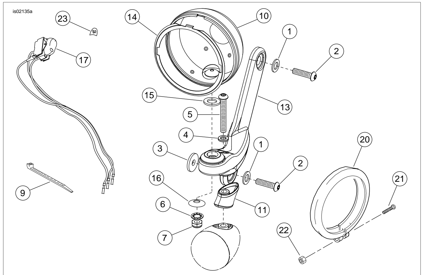
Figure 8. Service Parts: Custom Auxiliary Forward Lighting Kit
